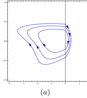
FIGURE 4. (a) The three limit cycles of the discontinuous piecewise differential system (25)–(26).
