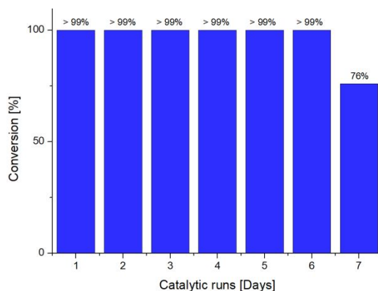
Figure 1 Recyclability experiments for the isomerization of 1-octen-3-ol to 3-octanone catalyzed by Ru@dendrimer 17 for seven consecutive runs.
