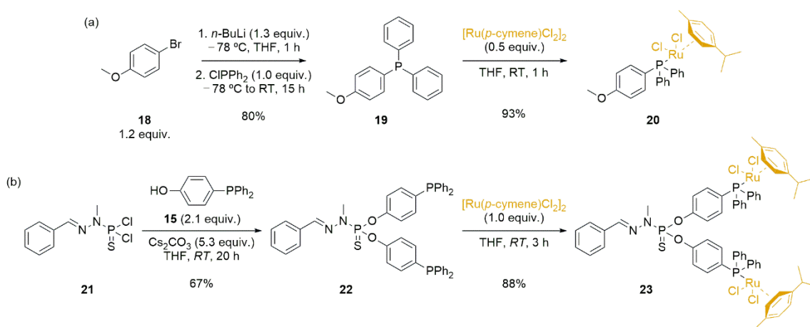
Scheme 4 Synthesis of Ru-complexes 20 and 23 , monometallic and bimetallic analogs of the Ru@dendrimer 17 , respectively.
