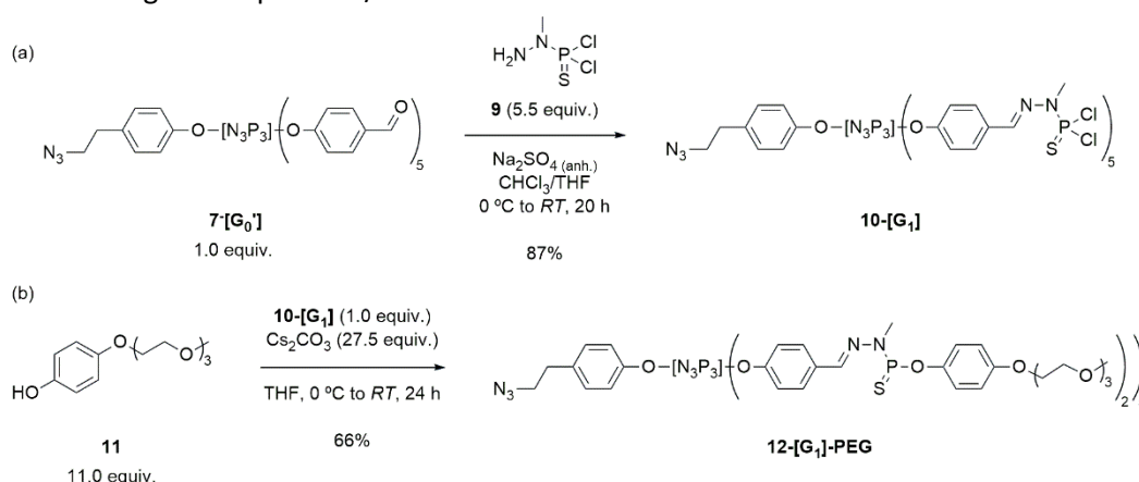
Scheme 2 Synthesis of (a) the first-generation azide dendron 10-[G 1 ] , and (b) its PEG-surface modified 12-[G 1 ]-PEG dendron.
