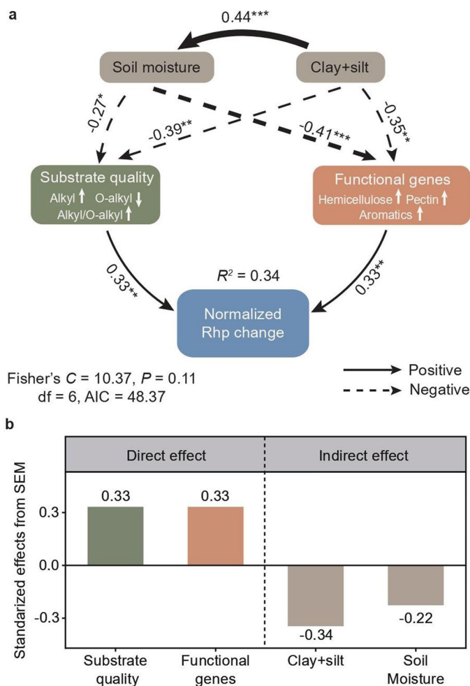
Extended Data Fig. 10 | Effects of abiotic and biotic factors on the normalized potential heterotrophic respiration (Rhp) change. a , Structural equation model (SEM) of the direct and indirect pathways that affect the normalized Rhp change. b , Standardized direct effects of substrate quality and the abundances of microbial functional genes and the indirect effects of edaphic variables (clay+silt and soil moisture) on the normalized Rhp change. Solid and dotted arrows represent positive and negative relationships, respectively. Arrow width is proportional to the strength of the relationship. The numbers adjacent to the arrows denote standardized path coefficients. Substrate quality
