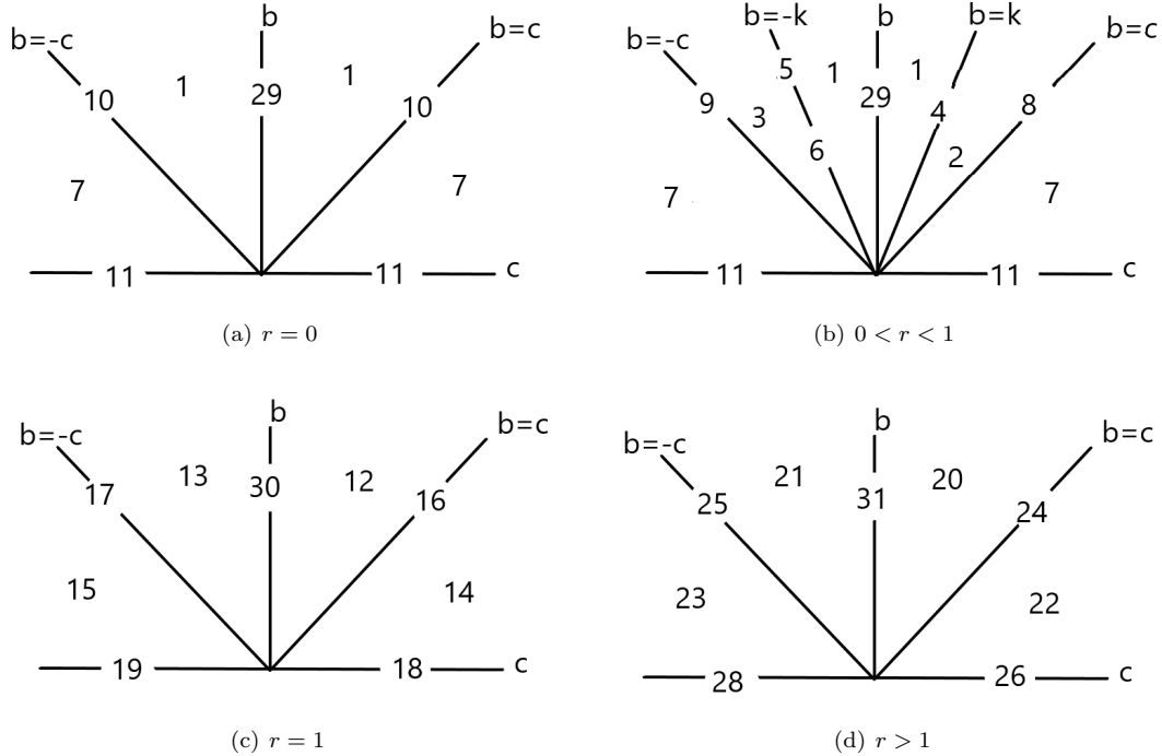
Figure 32. The bifurcation diagrams for the system (3) with e = 1 and b^2 + c^2 \neq 0 . Here k = c/\sqrt{1-r^2} . The number x denotes the phase portrait (x) for the values of the parameters b and c in the region or in the straight line where this number appears.
