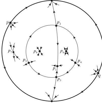
Figure 5. Local phase portrait in the Poincaré disc for case (I1) when b^2(r^2 - 1) + c^2 < 0 and b, c > 0 .
