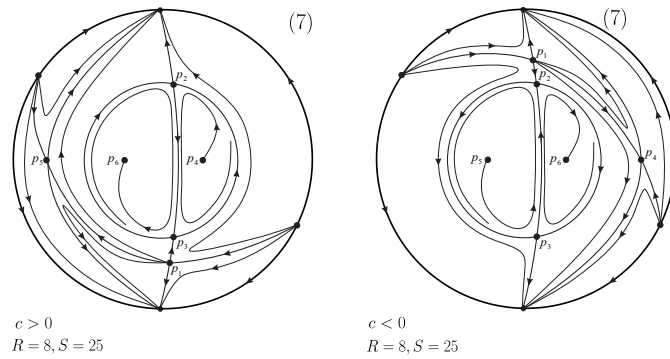
Figure 10. Global phase portraits in the Poincaré disc for case (II).
