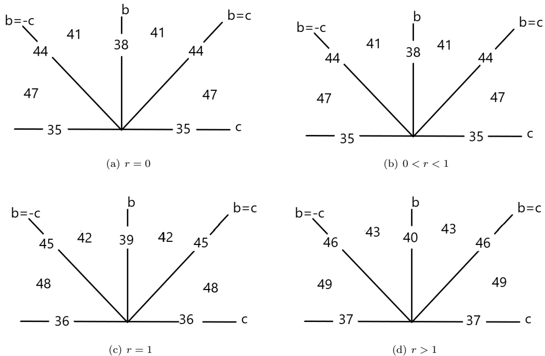
Figure 33. The bifurcation diagrams for the system (3) with e = 0 and b^2 + c^2 \neq 0 . The number x denotes the phase portrait (x) for the values of the parameters b and c in the region or in the straight line where this number appears.
