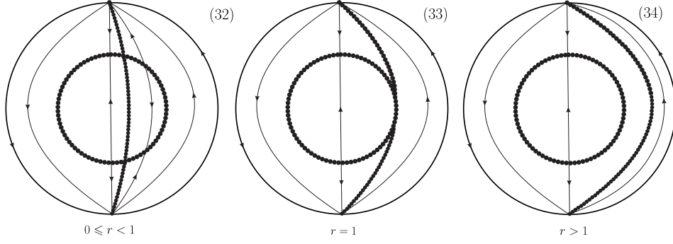
Figure 26. Global phase portraits in the Poincaré disc for case e = 1 , c = 0 and b = 0 .
