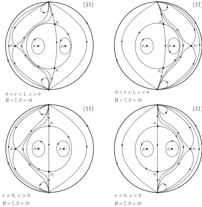
Figure 15. Global phase portraits in the Poincaré disc for case (IV).
