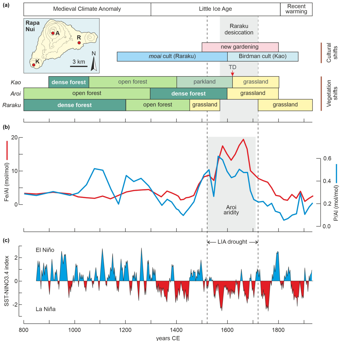
FIGURE 1 Last-millennium climatic, ecological and cultural shifts on Easter Island with emphasis on the Little Ice Age (LIA) drought bracketed by dashed lines (climatic phases after Nunn, 2007). (a) Summary of vegetation and cultural developments mentioned in the text (Rull, 2021). A, Aroi mire; K, Lake Kao; R, Lake Raraku; TD, total island deforestation. (b) Elemental ratios demonstrating the desiccation of the Aroi mire (Roman et al., 2021). (c) El Niño Southern Oscillation (ENSO) variability reconstruction using the normalized SST-NINO3.4 index (Delcroix et al., 2022).
