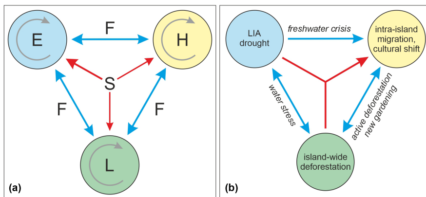
FIGURE 2 The Environment-Human-Landscape Feedbacks and Synergies (EHLFS) framework for socioecological analysis (a) and its application to the Little Ice Age (LIA) drought that occurred on Rapa Nui (b). E, environment; H, humans; L, landscape; F, feedbacks; S, synergies. Modified from Rull and Stevenson (2022).
