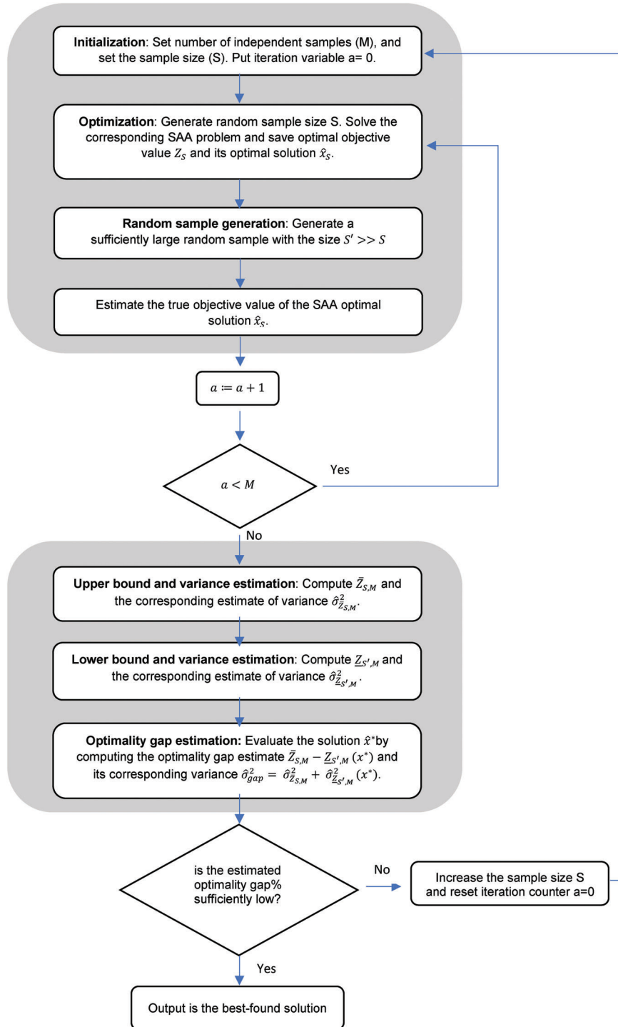
Fig. 2. Flowchart of the SAA algorithm.
