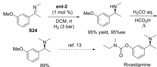
Figure 4. Assessment of isolated catalyst 2 in the asymmetric hydrogenation of different imines. Conversions are 100% as determined by 1 H NMR.
