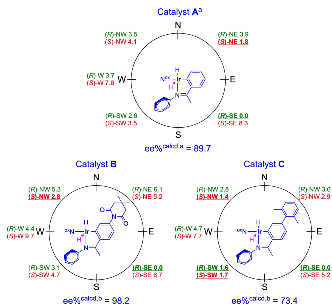
Scheme 3. DFT computed quadrant model for the hydrogenation of acetophenone N -methyl imine with catalyst containing cyclometallated imine A , B and C . Transition state relative \Delta\Delta G_{\text{DCM}}^{\ddagger} values for different orientations of the substrate phenyl group (in green: TSs leading to R isomer; in red: TSs leading to S isomer). The hydride transferred to the substrate is highlighted in magenta. The competitive TSs are highlighted in bold and underlined. Computed ee% over the complete set of TSs are reported for catalysts A , B and C (bottom). [a] Values adapted from [7] for the R enantiomeric series. [b] This work, values computed at B3LYP-D3/def2-TZVP, def2-QZVP(Ir)/SMD(DCM)//B3LYP-D3/6-31G(d,p), SDD + f(Ir)/SMD(DCM) considering the complete set of 5 pro- S and five pro- R TSs.
