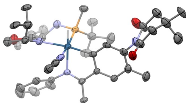
Figure 3. X-ray structure of 2 . The Ortep diagram shows ellipsoids at 50% probability. Only the H attached to iridium is drawn. TfO counterion and a co-crystallized DCM solvent molecule are omitted for clarity.
