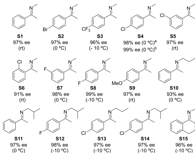
Figure 2. Results for the hydrogenation of N -methyl and N -alkyl imines using cyclometallating agent D . The catalyst was pre-formed in situ. Hydrogenation reactions were run overnight in DCM at 3 bar of H 2 with 1 mol % of catalyst at the temperature listed. 100% conversion was obtained in all cases, as determined by 1 H NMR. Enantiomeric excess was determined by chiral HPLC or GC of the corresponding trifluoroacetamide. a) Gram-scale reaction. b) Using cyclometallating agent E .
