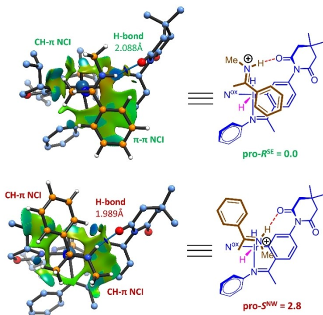
Figure 1. Comparison of the NCIs for the two lowest transition states for the hydrogenation of acetophenone N -methyl imine with catalyst B . NCIs are represented as blue (strong), green (weak) and red (repulsive) surfaces. \Delta\Delta G_{\text{DCM}}^{\ddagger} values are given in kcal·mol -1 .
