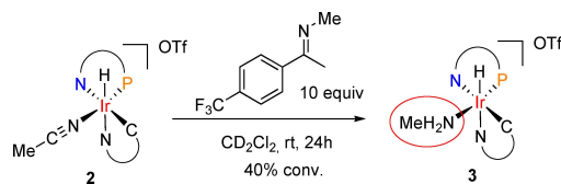
Scheme 5. In a stability test catalyst 2 was incubated in CD 2 Cl 2 solution with 10 equiv. of N -methyl imine substrate.
