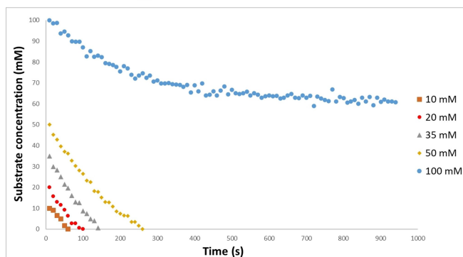
Figure 5. Kinetic profile of the hydrogenation of 4'-(trifluoromethyl)acetophenone N -methyl imine by 19 F NMR. Disappearance of starting imine plotted against time. The temperature of the NMR probe was constant at 37 °C. [2] = 0.2 mM for all experiments. [imine] = 10, 20, 35, 50 and 100 mM.
