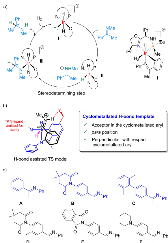
Scheme 2. a) Imine hydrogenation mechanism with Ir-P,N catalysts. b) Model transition state and H-bond acceptor. c) Cyclometallating agents used in the computational model (blue) and in the experimental study.
