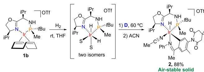
Scheme 4. Synthesis of cyclometallated catalyst 2 .
