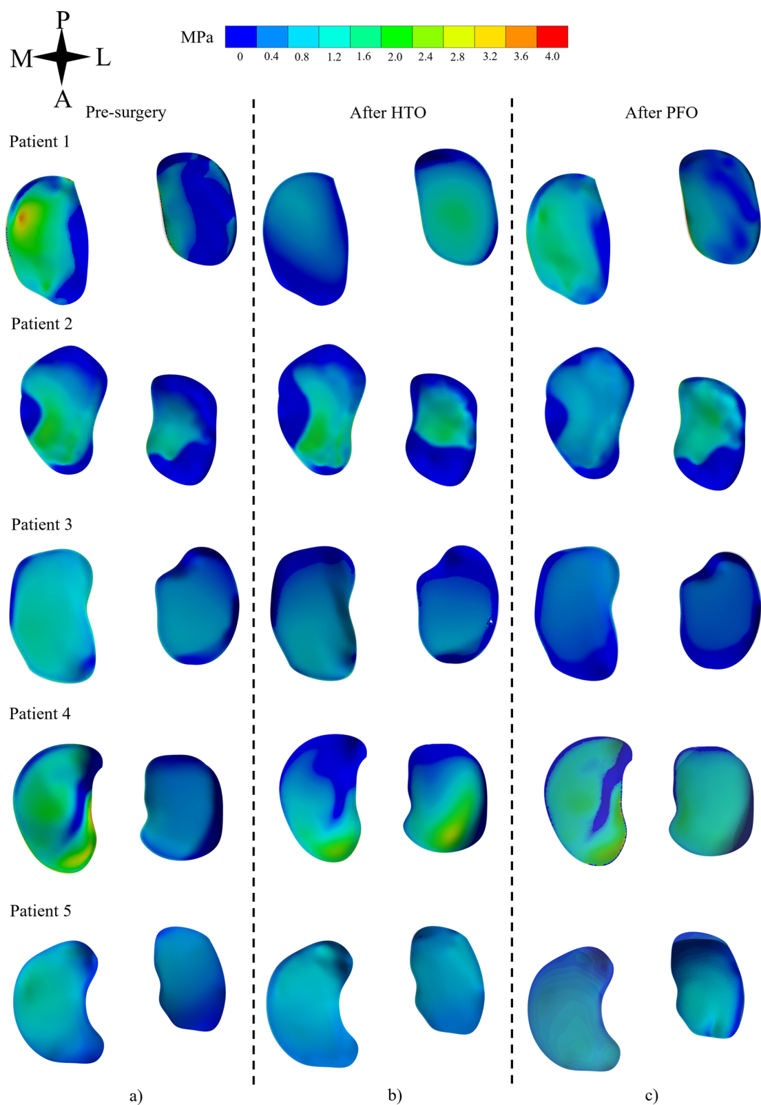
Fig. 4 Pressure distribution at the tibial plateau-cartilage contact interface, a before the surgery, b post HTO and c after PFO. M medial, L lateral, P Posterior, A Anterior
