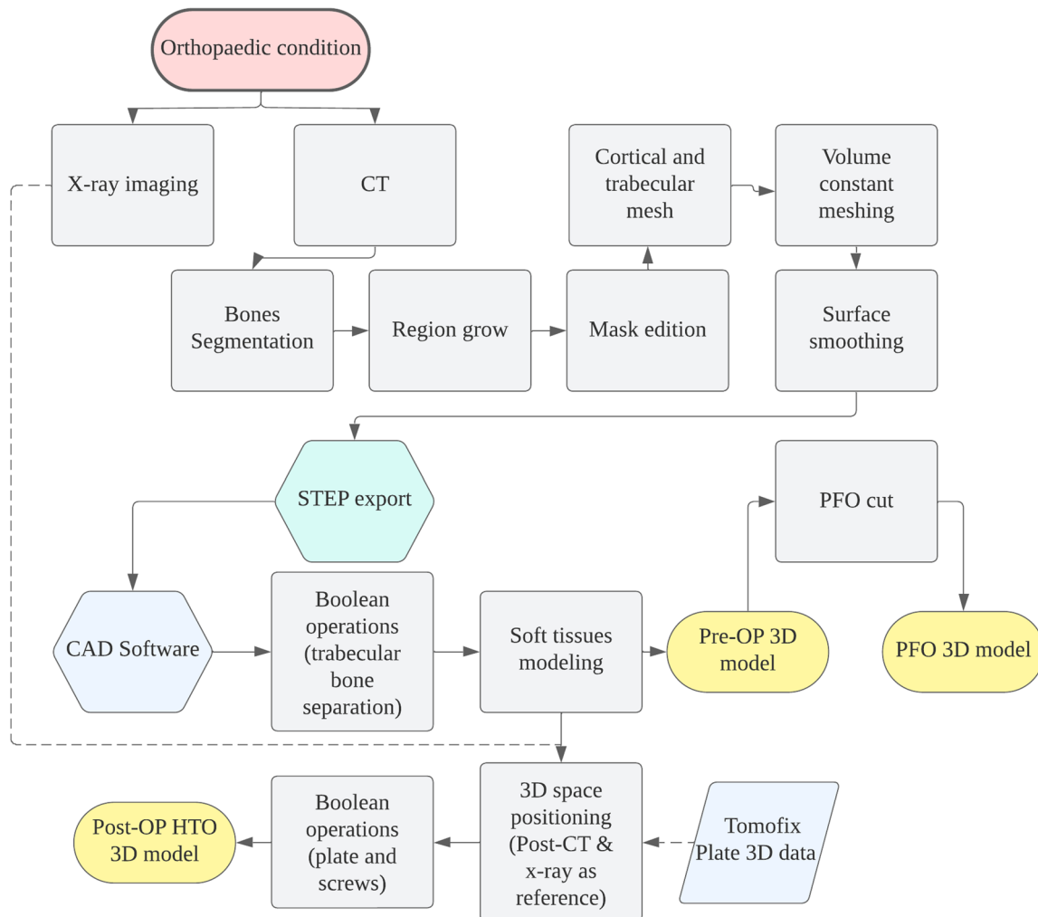
Fig. 6 Pre surgery (original), in-silico PFO, and post HTO model construction methodology
