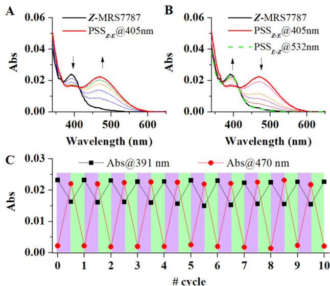
Figure 4. Photochemical characterization of MRS7787. (A) Variation of the absorption spectra of Z-MRS7787 in PBS:DMSO 98:2 upon irradiation at 405 nm (30 s increments at 6.5 \text{ mW cm}^{-2} ) and until a photostationary state ( \text{PSS}_{\text{Z-E}} ) is obtained ( c_{\text{MRS7787}} = 71 \mu\text{M} ). (B) Variation of the absorption spectra of the \text{PSS}_{\text{Z-E}} of MRS7787 in PBS:DMSO 98:2 upon illumination at 532 nm (60 s at 10 \text{ mW cm}^{-2} ) ( c_{\text{MRS7787}} = 71 \mu\text{M} ). For sake of comparison, the spectrum of the initial Z-MRS7787 compound is shown, which matches the spectrum of the \text{PSS}_{\text{E-Z}} achieved after irradiation at 532 nm. (C) Absorbance variation at 391 ( \lambda_{\text{max,Z-MRS7787}} ) and 470 nm ( \lambda_{\text{max,E-MRS7787}} ) upon 10 consecutive cycles of Z-E photoisomerization of MRS7787 in PBS:DMSO 98:2 under sequential irradiation at 405 nm (30 s at 6.5 \text{ mW cm}^{-2} ; violet) and 532 nm (60 s at 10 \text{ mW cm}^{-2} ; green) ( c_{\text{MRS7787}} = 71 \mu\text{M} ).
