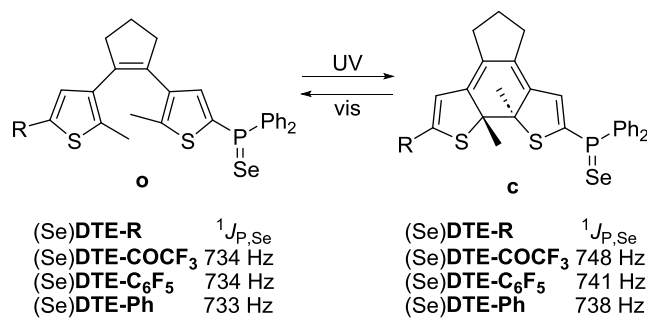
Scheme 4. Variation of ^1J_{\text{P,Se}} in the Open and Closed Isomers of the Selenides of \text{DTE-COCF}_3 , \text{DTE-C}_6\text{F}_5 , and \text{DTE-Ph}
