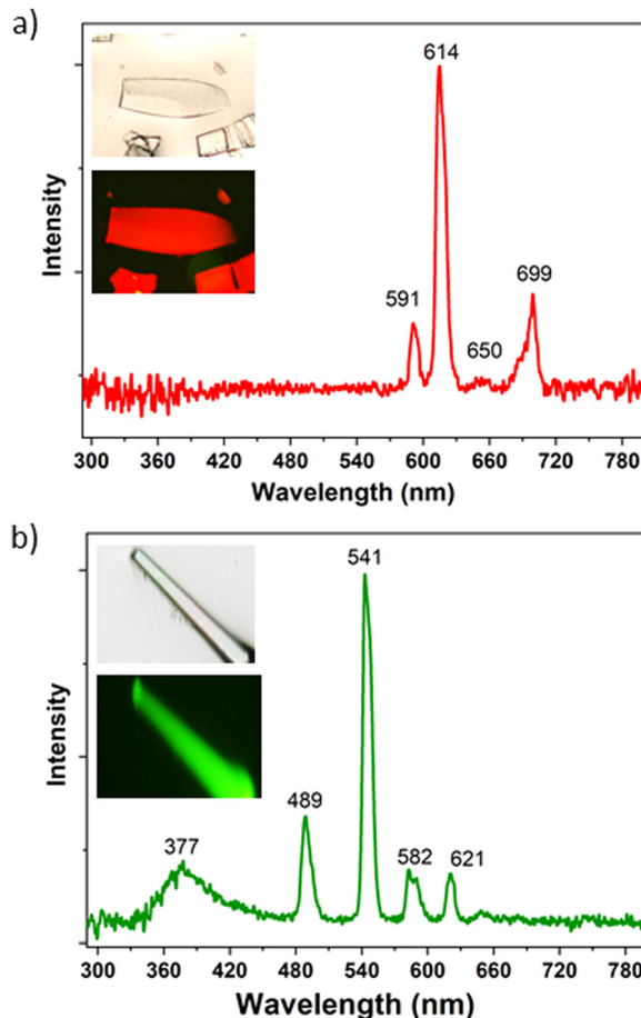
Fig. 3 Solid-state emission spectra of TDCA- \text{Eu} (a) and TDCA- \text{Tb} (b) under continuous-wave irradiation ( \lambda_{\text{ex}} = 290 nm) at room temperature. Insets: Optical microscopy images of the corresponding crystals under white and the corresponding luminescence images.
