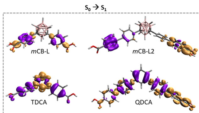
Fig. 2 Schematic diagrams for the energy absorption on photoexcitation from singlet states ( S_0 to S_1 ). Purple (negative values) and pale brown (positive values) lobes represent the electron density differences between the initial and final state calculated at STEOM-DLPNO-CCSD level.
