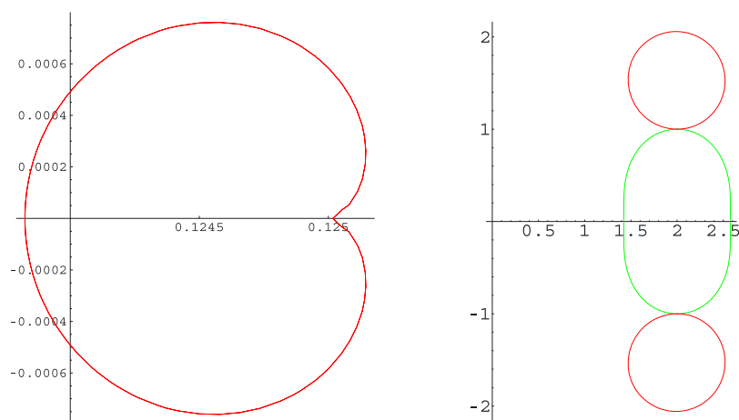
Fig. 4. Stability regions for z = 1 , z_1 and z_2 under the operator (4). (For interpretation of the references to colour in this figure legend, the reader is referred to the web version of this article.)
