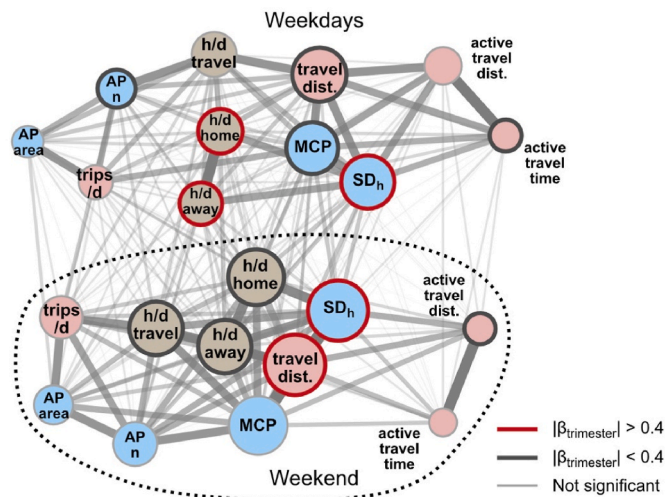
Fig. 6. Network illustration with activity space variables as nodes and their Spearman's rank correlations as edges (more correlated variables are closer together). The size and opacity of edges are proportional to the correlation between the nodes they connect and the size of nodes is proportional to their sum of absolute correlations. The node outline represents the association with trimester (black: significant association with an absolute coefficient >0.4 , dark grey: significant association with an absolute coefficient <0.4 , light grey: not significant association ( p > 0.05 )).
