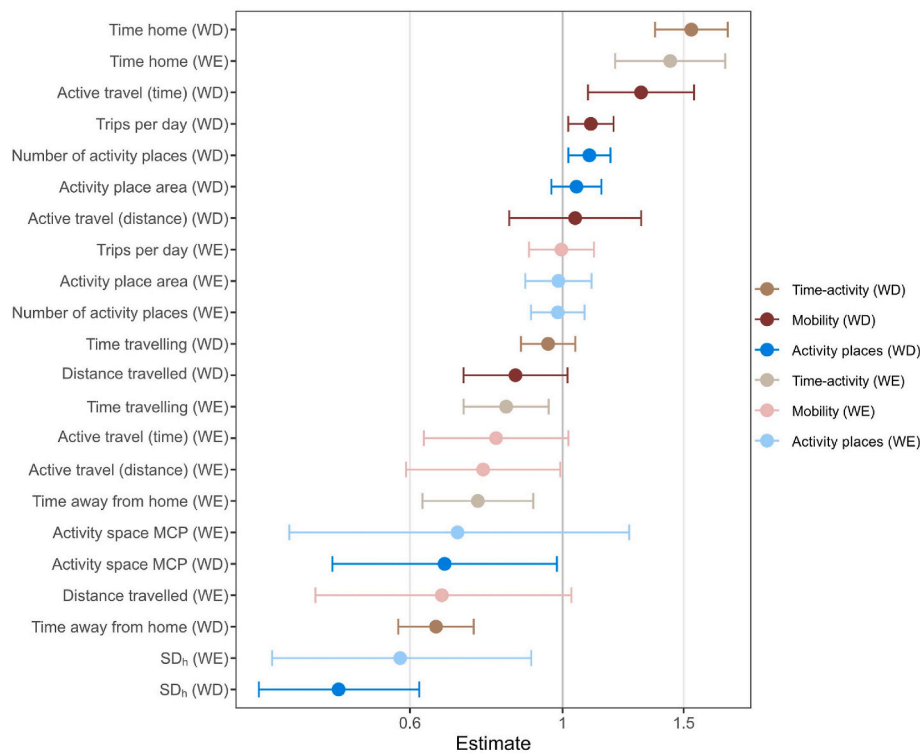
Fig. 4. Exponentiated regression coefficients of T3 with activity space variables as outcomes. Error bars represent 95% confidence intervals. MCP = minimum convex polygon. SD h = standard distance from home.
