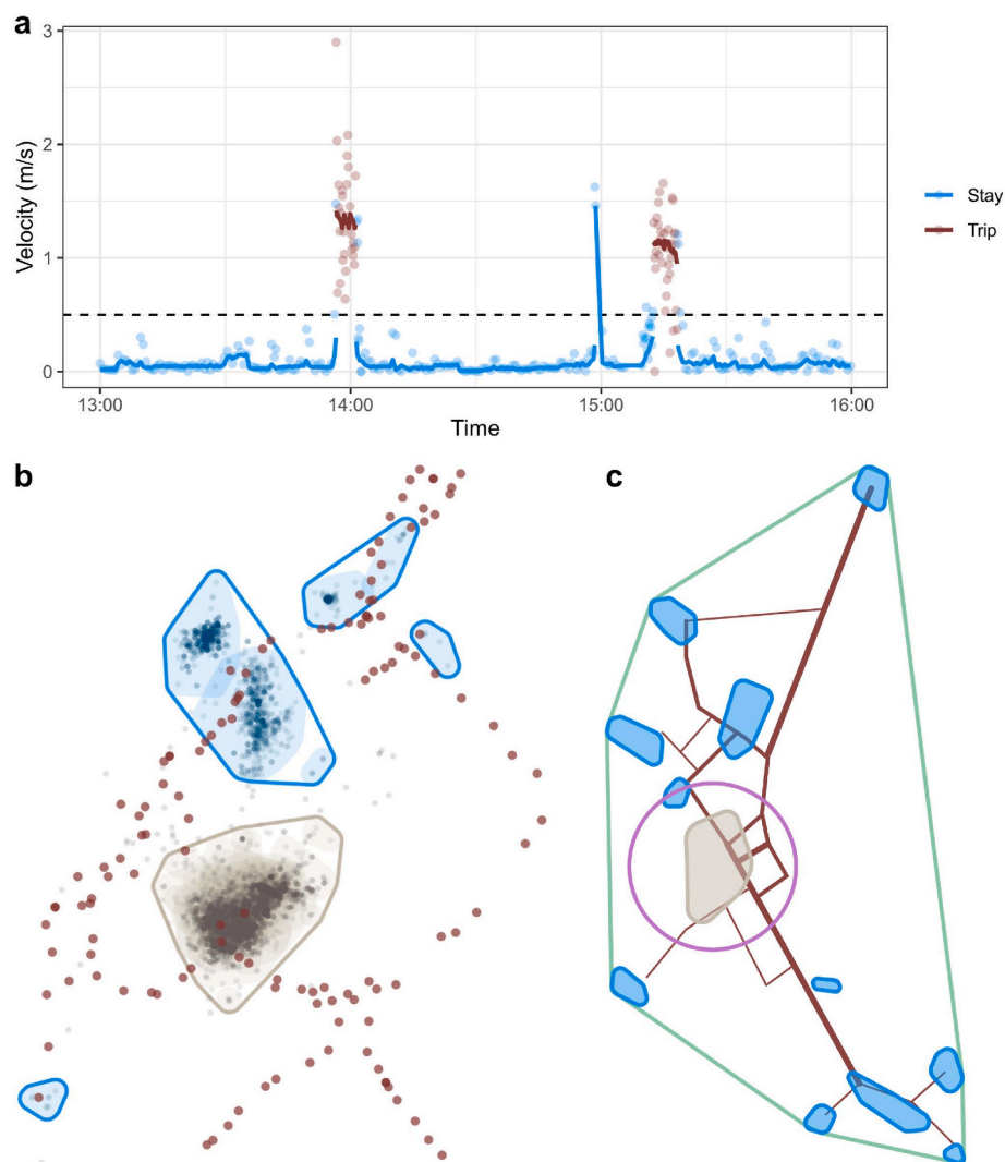
Fig. 2. a) Example of how GPS points were divided into stays and trips based on 3-min sliding windows. Lines show 3-min means. At least three consecutive points with 3-min mean velocity >0.5 m/s (dashed line) were classified as a trip. Note two points around 15:00 that were not classified as a trip. b) GPS points belonging to stays (small points) were clustered into stay geometries (translucent polygons) that were further grouped into activity places (solid polygon boundaries). The activity place coded as home is coloured grey, with remaining activity places in blue. GPS points belonging to trips are shown in red. c) Schematic illustration of an activity space. Eleven activity space variables were calculated: 1) time staying at or near home (grey polygon), 2) time staying away from home (blue polygons), 3) time travelling (red lines), 4) number of trips per day, 5) kilometres travelled per day, 6) active travel distance ratio, 7) active travel time ratio, 8) number and 9) area of activity places (grey and blue polygons), 10) activity space MCP (green boundary), 11) time-weighted standard distance from home (the radius of the purple circle).
