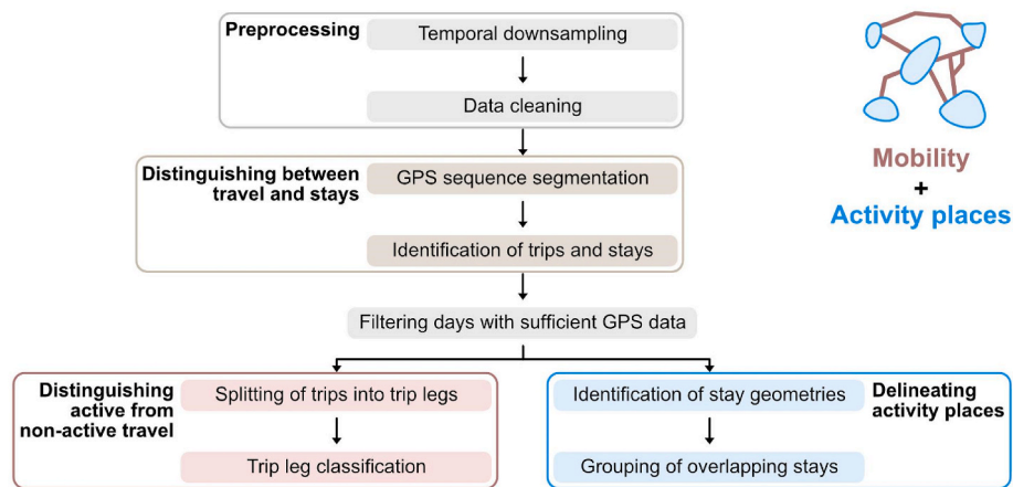
Fig. 1. The sequence of steps in ActMAP.
