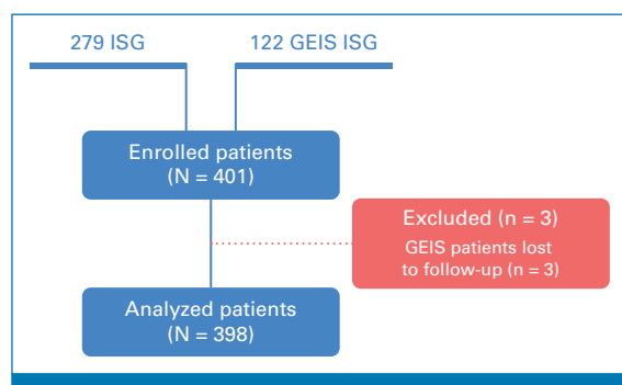
FIG A2. Study flow diagram of the combined analysis of the Italian ISG/OS-2 and Spanish GEIS-33 studies.
