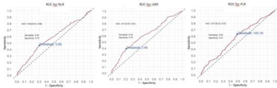
Figure1. ROC curves for NLR, LMR and PLR and 5-year survival.
