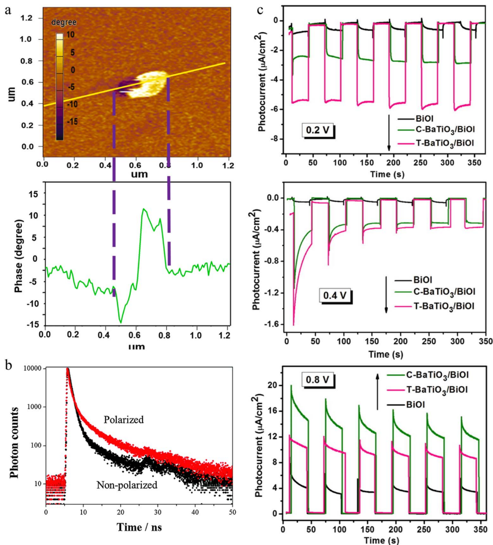
Fig. 12 (a) Phase maps (top) and corresponding curve (bottom) of the piezoelectric response. 255 Copyright © 2018 Elsevier. (b) Decay profile of PL from K 0.5 Na 0.5 NbO 3 . 314 Copyright © 2014 Royal Society of Chemistry. (c) Transient photocurrent responses at different bias voltages. 67 Copyright © 2017 Elsevier.
