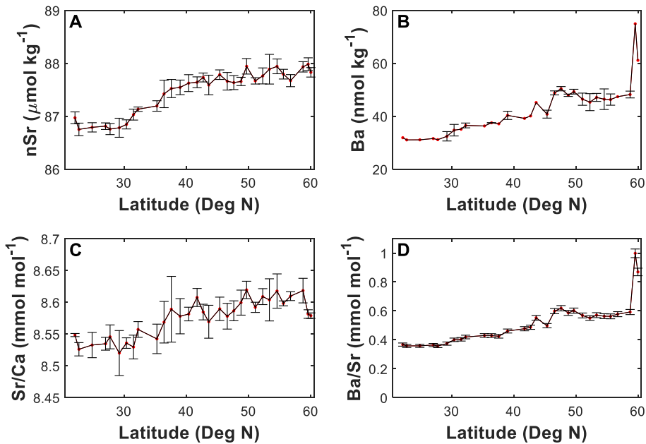
Fig. 3. Surface water concentrations along the Hawaii to Alaska transect (samples collected 2–5 m below the sea surface).
