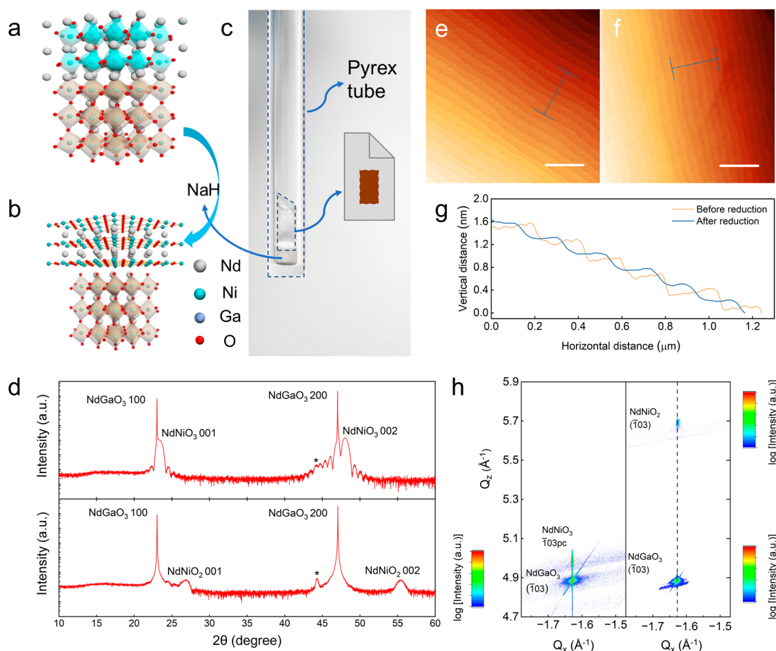
Figure 1. Structural characterization of \text{NdNiO}_3 and \text{NdNiO}_2 films on (001)_{\text{pc}} -oriented \text{NdGaO}_3 substrates. Schematic crystal structure of (a) \text{NdNiO}_3 grown on \text{NdGaO}_3 and (b) \text{NdNiO}_2 on \text{NdGaO}_3 . After reduction using \text{NaH} , the structure changes from perovskite to the infinite-layer phase. (c) Optical image of the Pyrex tube with the sample wrapped in aluminum foil and \text{NaH} powder inside the tube. (d) Specular \theta – 2\theta scans around the 001 and 002 peaks of the \text{NdGaO}_3 substrate for the \text{NdNiO}_3 film (top) and the \text{NdNiO}_2 film (bottom). * denotes the unfiltered parasitic peak from the diffractometer. Upon topochemical reaction, the out-of-plane parameter changes from 3.787 to 3.315 Å. (e, f) AFM topography of thin films before and after reduction, respectively. The scale bars represent 1 \mu\text{m} . (g) The line profile of thin films before and after reduction. (h) Reciprocal space maps around the \bar{1}03 peak of the \text{NdGaO}_3 substrate for the \text{NdNiO}_3 film (left) and the \text{NdNiO}_2 film (right). Each map was completed through multiple scans.
