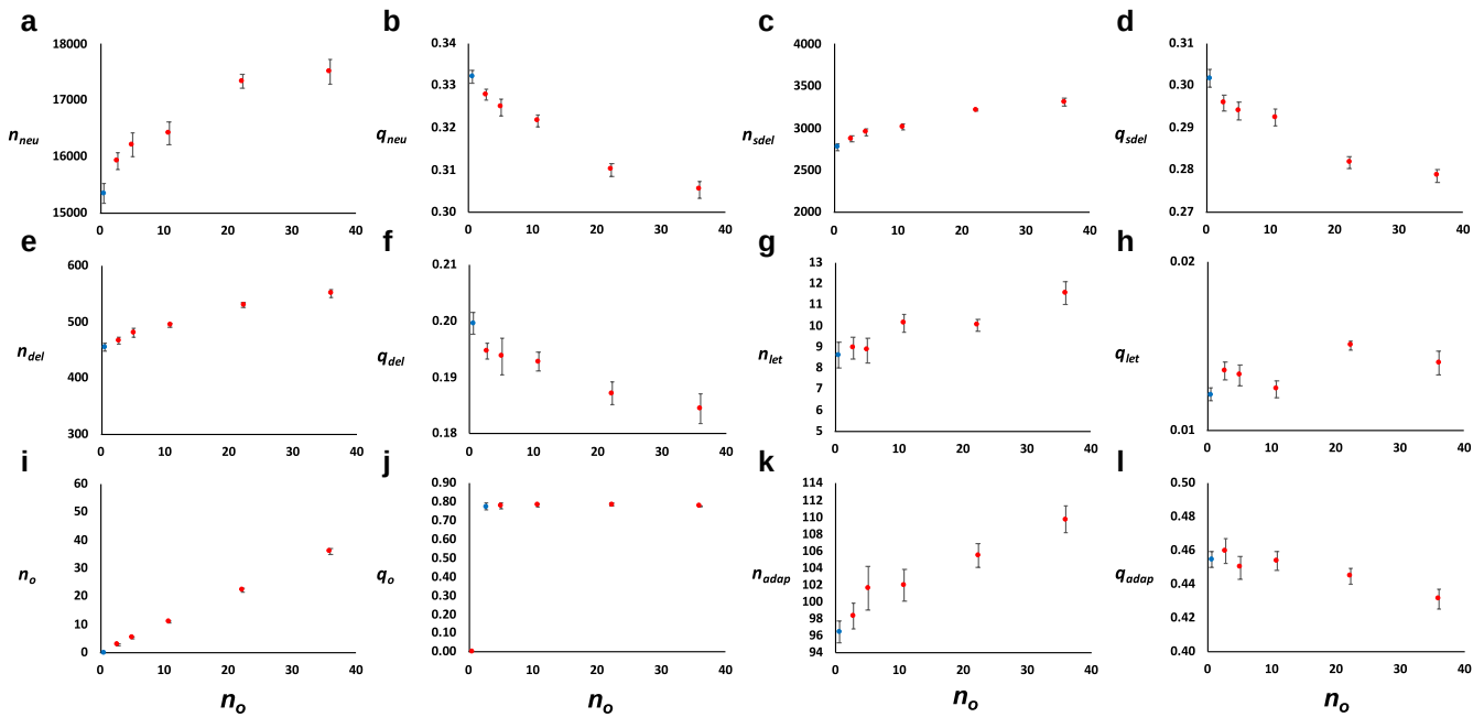
Fig. 6. Mean number ( n ) and average frequency ( q ) of neutral (subscript neu , panels a, b), partially recessive deleterious ( del , panels e, f), additive slightly deleterious ( sdel , panels c, d), lethal ( let , panels g, h), adaptive ( adap , panels k, l), and overdominant ( o , panels i, j) mutations. Results refer to simulations that assume an ancestral effective population size of N_e = 10^4 . The blue dots (first from left-hand side in each panel) correspond to the simulation results assuming the mutation model M1S without overdominance, which parameters are shown in Table 1. The red dots refer to the models assuming the same parameters as for model M1S but also including overdominant mutations at a rate ( U_o ) ranging from 0.5 \times 10^{-7} to 8 \times 10^{-7} , with the x-axis indicating the mean number of overdominant segregating mutations ( n_o ) for each overdominance mutation rate. Results are based on 10 simulation replicates and bars indicate 95% confidence intervals.
