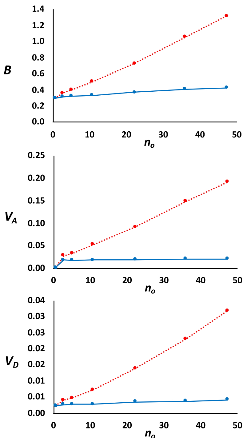
Fig. 7. Changes of inbreeding load ( B ), additive variance ( V_A ) and dominance variance ( V_D ) for models assuming the same parameters as for model M1S (parameter in Table 1), but also including overdominant mutations occurring at different rate U_o , leading to different numbers of segregating overdominant mutations ( n_o ). Results refer to simulations that assume an ancestral effective population size of N_e = 10^4 . Red dots and dotted lines give the overall values contributed for all kind of loci, with the x-axis indicating the mean number of overdominant segregating mutations ( n_o ) for each overdominance mutation rate. Blue dots and continuous lines indicate the contribution from segregating nonoverdominant loci. Results are based on 10 simulation replicates.
