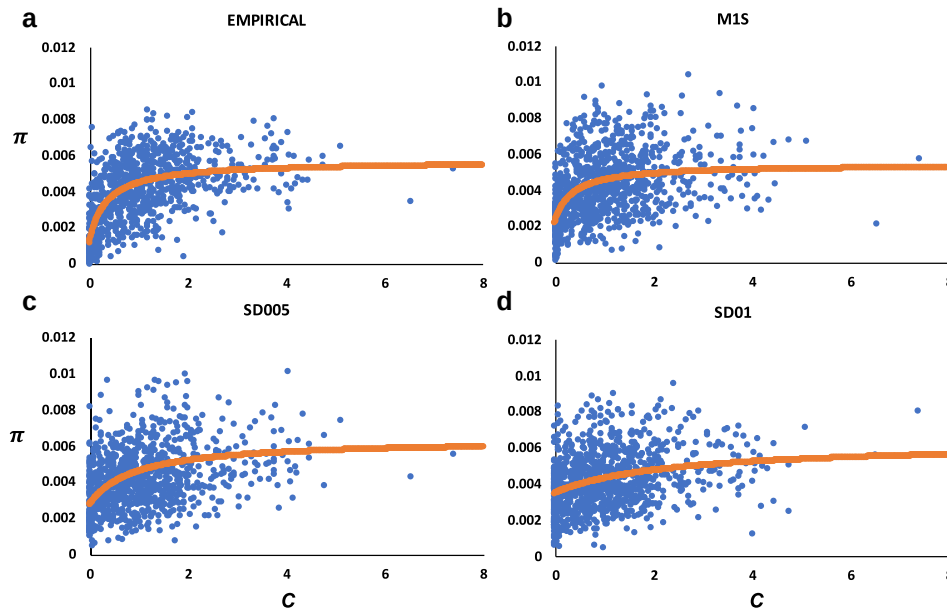
Fig. 4. Relationship between the mean nucleotide diversity ( \pi ) and the mean recombination rate ( c ) in centimorgans (cM) per megabase (Mb) for 100-kb genomic windows considering the 4 autosomal chromosome arms, for simulation which assume an ancestral effective population size of N_e = 10^5 . The curve shown in each graph represents the rational function fitted to the data. a) Empirical data. b) Simulation results for model M1S without overdominant mutations. (c and d) Models assuming the same parameters as for model M1S and also including overdominant mutations at a rate ( U_o ), 0.05 \times 10^{-7} (SD005) and 0.1 \times 10^{-7} (SD01). Simulation data is based on the average of 3 replicates.
