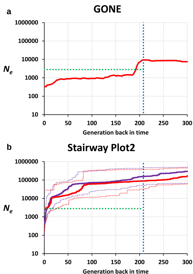
Fig. 1. Estimates of historical effective population size ( N_e ) obtained from linkage disequilibrium between SNPs (software GONE, panel a), or from the SFS of variants (software Stairway Plot2, panel b). For this latter, the thick lines are median values and the thin dotted lines are the 95% confidence limits, with purple lines denoting the results using the silent sites and red lines those using the synonymous sites. The vertical blue-dotted line indicates the time when the population was captured and maintained in the laboratory since then. The horizontal green-dotted line indicates the total number of individuals maintained in the laboratory population.
