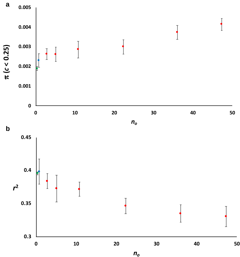
Fig. 5. Average nucleotide diversity ( \pi ; panel a) and linkage disequilibrium between consecutive loci ( r^2 ; panel b) for a range of simulated overdominant mutation rates, ranging from U_o = 0.5 to 8 \times 10^{-7} , with the x-axis indicating the mean number of overdominant segregating mutations ( n_o ) for each overdominance mutation rate. Results refer to simulations that assume an ancestral effective population size of N_e = 10^4 . The values of \pi refer to 100-kb genomic windows with average recombination rate c < 0.25 cM/Mb. Dots indicate the mean \pi or r^2 based on the 10 simulated replicates, and bars indicate the 95% confidence intervals. The green dots (first from the left-hand side) refer to the empirical data with confidence limits obtained by bootstrapping, the blue dots (second from the left-hand side) correspond to the simulation results assuming the mutation model M1S without overdominance, which parameters are shown in Table 1. The remaining red dots refer to the models assuming the same parameters as for model M1S but also including overdominant mutations at a rate ( U_o ) ranging from 0.5 \times 10^{-7} to 8 \times 10^{-7} .
