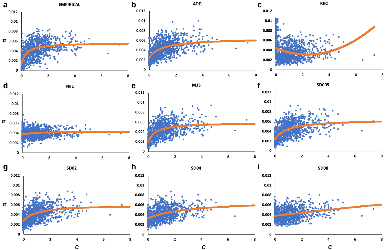
Fig. 2. Relationship between the mean nucleotide diversity ( \pi ) and the mean recombination rate ( c ) in centimorgans (cM) per megabase (Mb) for 100-kb genomic windows considering the 4 autosomal chromosome arms, for simulation that assume an ancestral effective population size of N_e = 10^4 . The curve shown in each graph represents the rational function fitted to the data (except for the REC model for which this function cannot be fitted and a polynomial curve is presented instead). a) Empirical data. (b–i) Simulation results without (panels b–e) or with (panels f–i) overdominant mutations. ADD, REC: all mutations are assumed to be additive or fully recessive, respectively. NEU: only neutral mutations are assumed. M1S: mutations assuming the parameters shown in Table 1. SD005–SD08: mutations assuming the same parameters as for model M1S and also including overdominant mutations at a rate ( U_o ), 0.5 \times 10^{-7} (SD005), 2 \times 10^{-7} (SD02), 4 \times 10^{-7} (SD04), 8 \times 10^{-7} (SD08). Simulation data is based on the average of 10 replicates.
