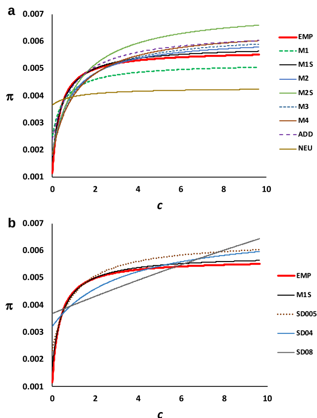
Fig. 3. Rational function fitted to the mean values of nucleotide diversity ( \pi ) with respect to the mean recombination rate ( c ) in centimorgans (cM) per megabase (Mb) for 100-kb genomic windows considering the 4 autosomal chromosome arms, for simulation that assume an ancestral effective population size of N_e = 10^4 . a) Empirical (EMP) data and models excluding overdominant mutations, as shown in Table 1. b) Empirical (EMP) data, model M1S excluding overdominant mutations, and models assuming the same parameters as for model M1S, and also including overdominant mutations at a rate ( U_0 ), 0.5 \times 10^{-7} (SD005), 4 \times 10^{-7} (SD04), 8 \times 10^{-7} (SD08).
