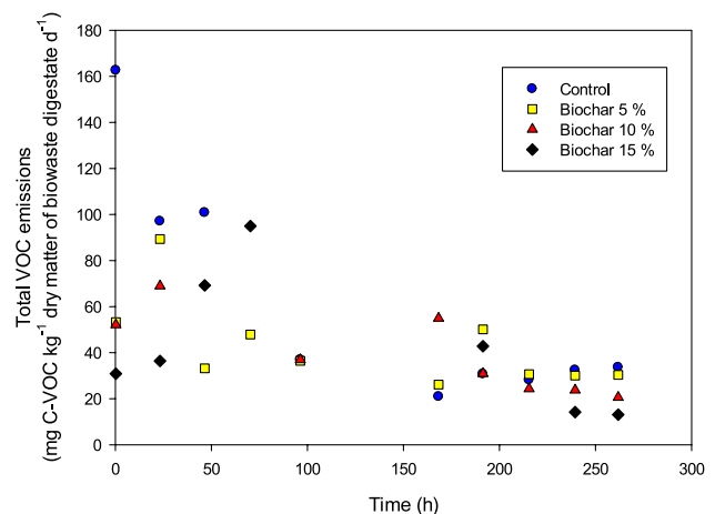
Fig. 5 Total VOC specific emission rate during the composting process of biowaste digestate at different ratios of biochar
