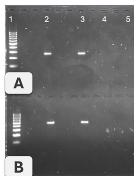
Fig. 6 Agarose gel electrophoresis of double-tagged PCR amplicons obtained using a conventional benchtop thermocycler and a handheld battery-operated thermocycler (miniPCR®). Panel A shows amplification of the IS6110 target and panel B the gyrB target. In both panels, lane 1 corresponds to the molecular weight marker, lane 2 to the positive sample amplified with the benchtop thermocycler, lane 3 to the positive sample amplified with the miniPCR®, lane 4 to the negative control processed with the benchtop thermocycler, and lane 5 to the negative control processed with the miniPCR®. DNA from M. bovis BCG-Pasteur at 2.6 \times 10^7 CFU mL -1 was used as a positive sample, whereas negative controls were processed in parallel in the absence of template DNA.
