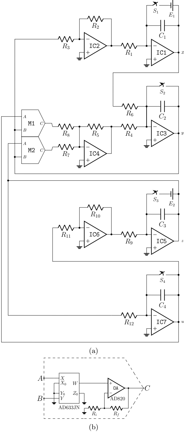
FIG. 4: Electronic circuit diagram and the multiplier embedded schematic.
