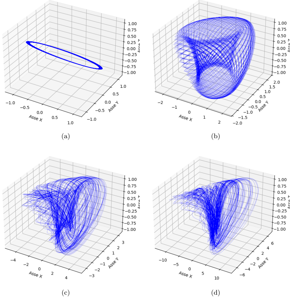
FIG. 5: Spice simulation representing the attractor in phase space x - y - z of Eqs. (4) at different value of \mu : 0.01, 0.4, 0.75, 1 respectively in Figs. 5a, 5b, 5c, 5d.
