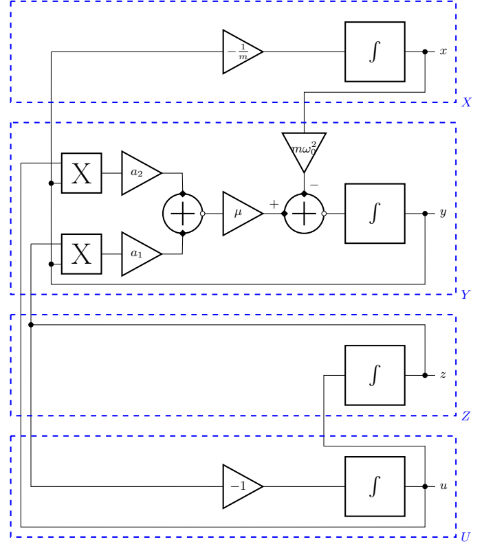
FIG. 3: Design block implementation of Eqs. (3). The architecture consists of four functional blocks X , Y , Z , U , each enclosed by a blue, dashed box, where it implements the differential equations providing x , y , z and u .
