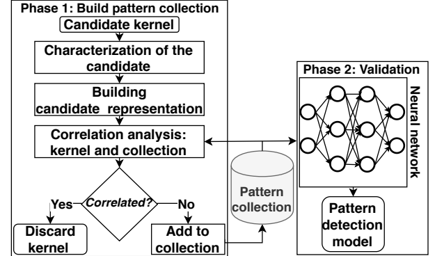
Fig. 4. Summary of the experimentation workflow.
