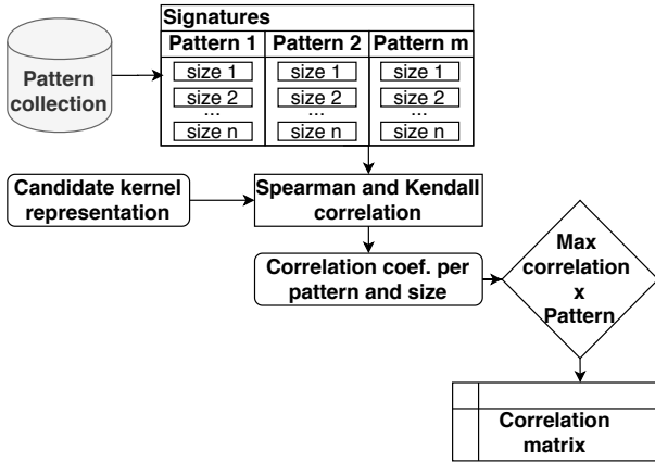
Fig. 3. Process for obtaining the correlation of the candidate kernel against the pattern collection .
