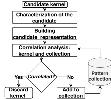
Fig. 1. Methodology for determining whether a pattern should be included or not in the training set.
