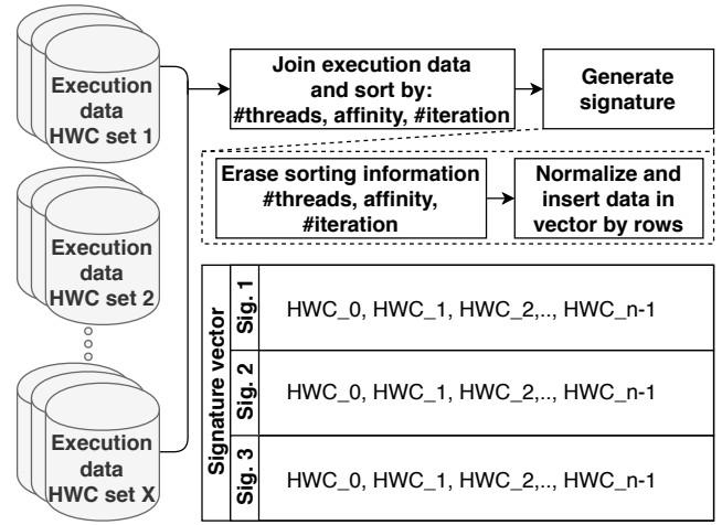
Fig. 2. Methodology to build the candidate kernel representation.
