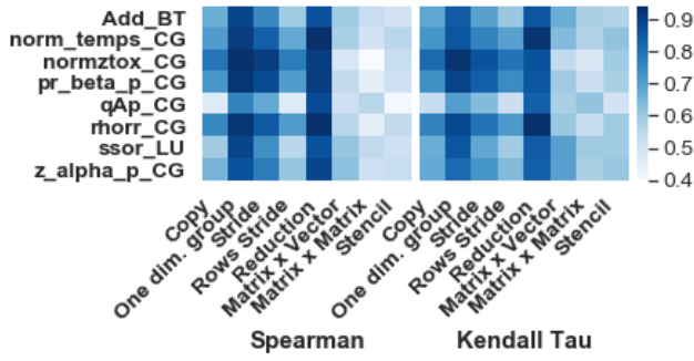
Fig. 7. Correlation coefficients between NPB extracted kernels and the pattern collection .
