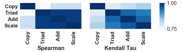
Fig. 5. Spearman and Kendall maximum correlation for STREAM kernels.
