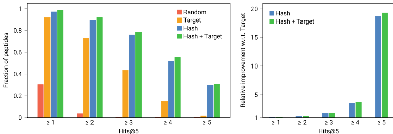
Fig. 3. Distribution of Hits@5 scores across evaluated models, showing hash-based models achieve higher frequencies of multiple correct predictions.
