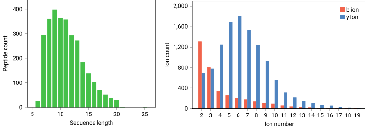
Fig. 2. Dataset composition showing sequence length distribution and b/y ion counts.
