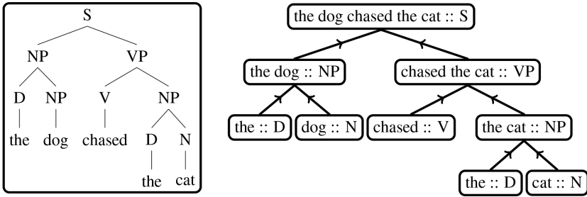
Figure 4. The equivalence of the representational and derivational construals of CFGs rests on allowing the entire derivation to “count”, as in Figure 2.
