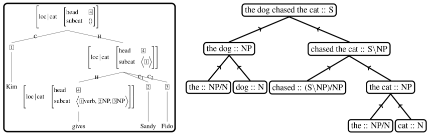
Figure 3. Taking categorial grammar as our derivational theory, it is very natural to adopt the view in Figure 2 rather than that in Figure 1.
