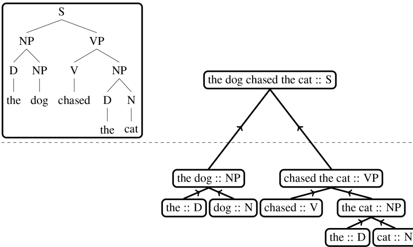
Figure 5. Restricting ourselves to understanding derivational theories as in Figure 1 would entail that the representational and derivational construals of CFGs were not equivalent.
