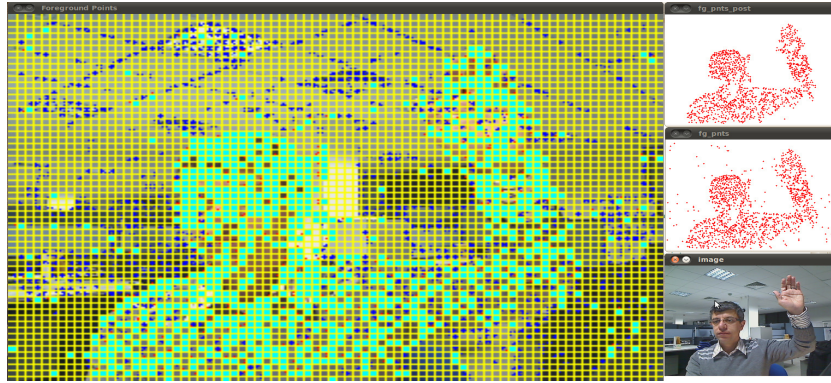
Figure 5: Left: foreground blocks, Right from down to top: the real image, foreground IPs before, and after post-processing.
