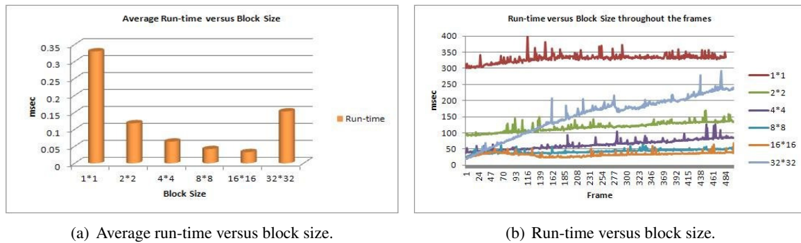
Figure 8: Run-time versus block size
