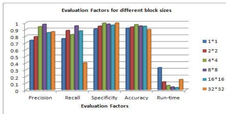
Figure 6: Evaluation Factors versus block sizes for resolution 512 \times 256 .
