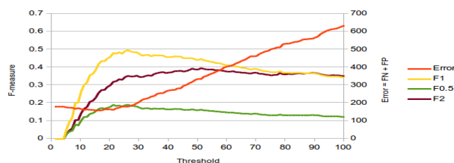
Figure 10: F-measure and total number of error versus threshold.
