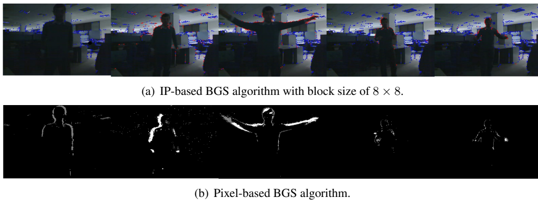
Figure 9: Comparison between IP-based and pixel-based BGS methods under low-light conditions over 5 random frames of a video with 450 frames.
