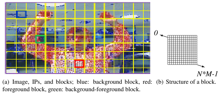
Figure 1: The block and its different types.
