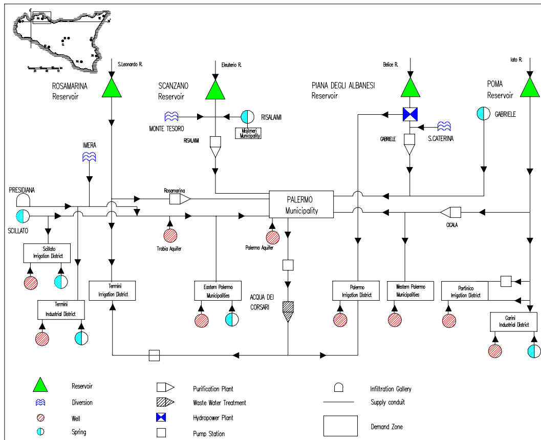
Figure 2. Scheme of the Palermo Water Supply System
