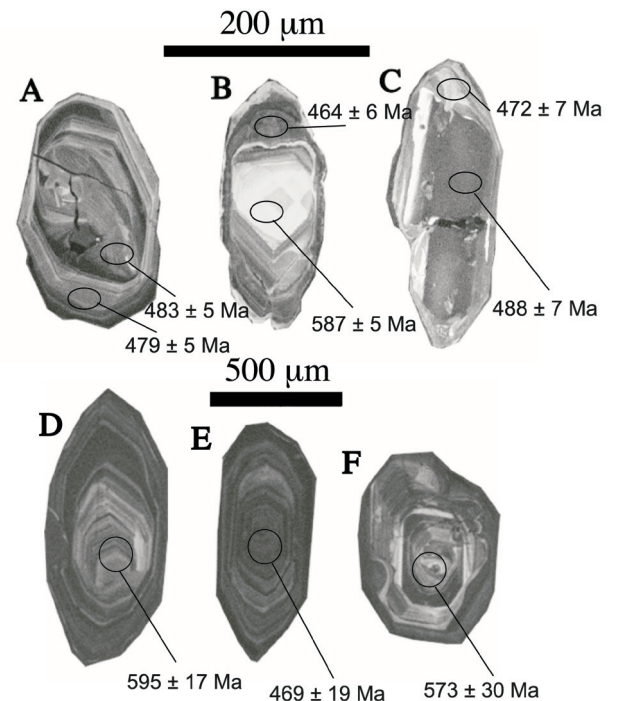
FIGURE 2 | Cathodoluminescence images of selected zircons from the Sisargas orthogneiss. A, B and C have been dated by ion microprobe and D, E and F have been dated by LA-ICPMS.
