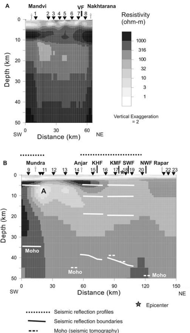
FIGURE 6 | Geoelectric structure obtained for both the profiles from 2-D inversion of magnetotelluric data using the non-linear conjugate gradient algorithm of Rodi and Mackie (2001) shown along with geological faults. Prominent reflection boundaries as well as Moho obtained from passive seismological tomography studies are plotted.
