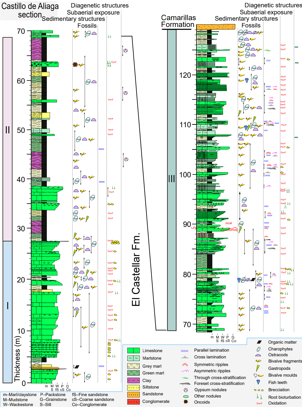
FIGURE 2. The El Castellar Formation in the Castillo de Aliaga section. Lithologic and textural log including the sedimentary structures, fossil content, subaerial exposure features, and diagenetic structures, as well as the three different stratigraphic sections (I, II and III) identified in the studied section.
