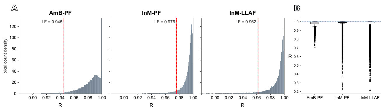
FIGURE 6. Maximum Roughness outlier detection. A) Density histograms of \bar{R} values for each DSM. The red line indicates the LF threshold used to identify Maxim Roughness outliers ( \bar{R} < LF ). B) Boxplots of \bar{R} values for each DSM, highlighting the distribution of Maximum Roughness outliers (black points), the blue line indicates Minimum Roughness outliers at \bar{R} = 1 .
