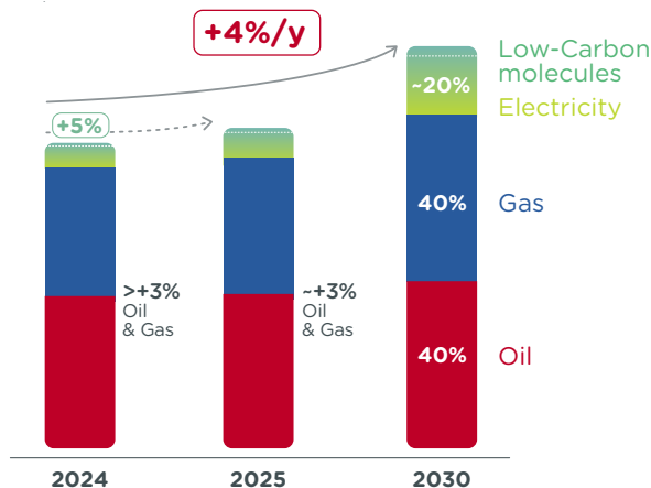
Energy Production (in PJ/d)
