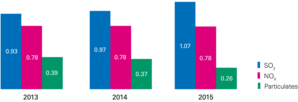
Specific emissions compared to total net production (g/kWh)
