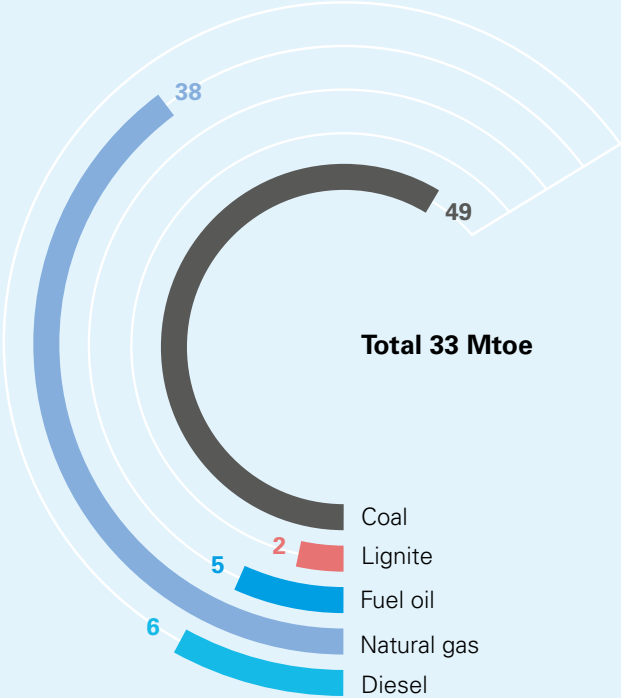
Consumption of fossil fuels for simple and combined thermal production 2017 (%)
