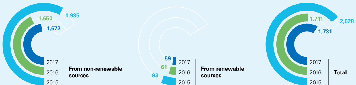
Fuel consumption by primary source (,000 TJ)
