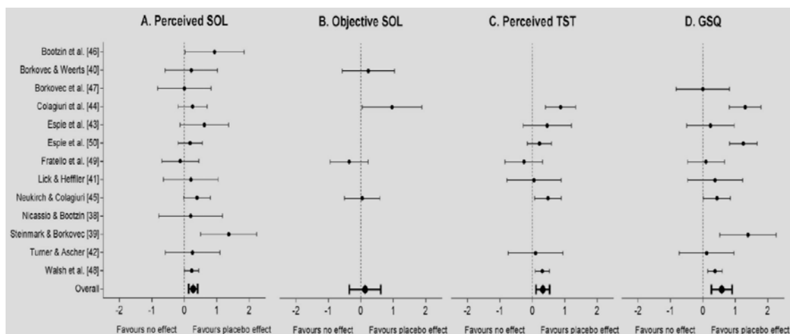
Fig. 2. Forest plots showing Hedge's g ( \pm 95\% CI) for individual studies and overall effects for A. perceived SOL, B. objective SOL, C. perceived TST, and D. perceived GSQ.
