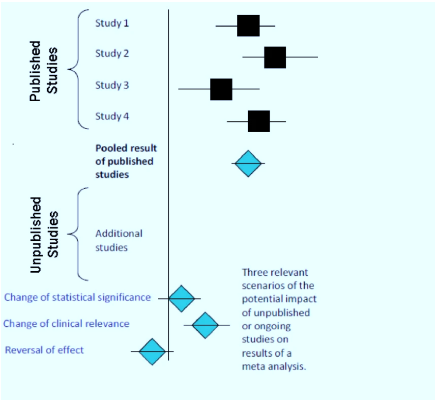
Figure 1: Schematic illustration of the potential impact of unpublished studies on a meta-analytic summary effect
