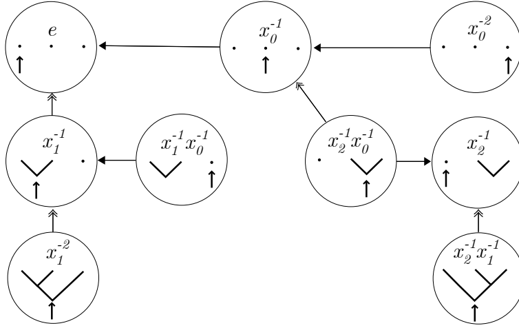
FIGURE 4. The negative forest NF(3)
