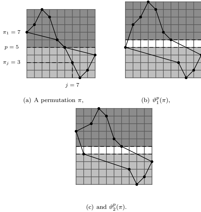
FIGURE 2. Example of the \vartheta -construction
