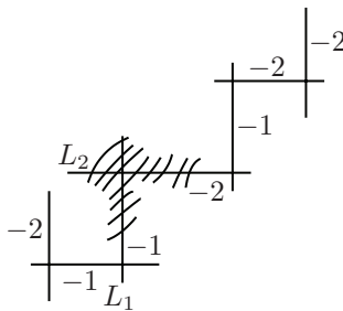
FIGURE 5.1. Configuration of the exceptional divisor.
