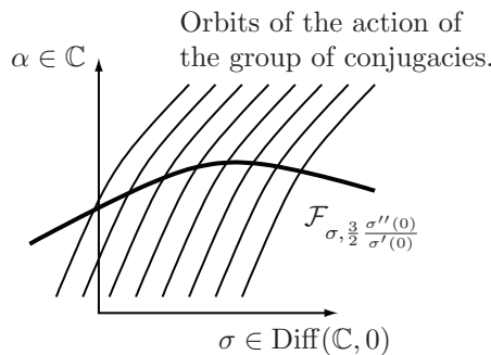
FIGURE 3.2. Moduli space of absolutely dicritical foliations.
