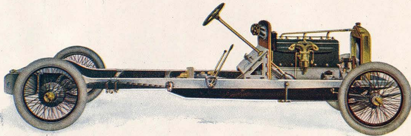
Chassis Minerva 30 HP (6 cylinders)
