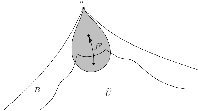
Figure 4.9: If the new set \tilde{U} left some neighbourhood of \alpha , there would be points in it stepping outside it under f^p . The shaded set represents the attracting petal attached to \alpha given by the Fatou coordinates.
