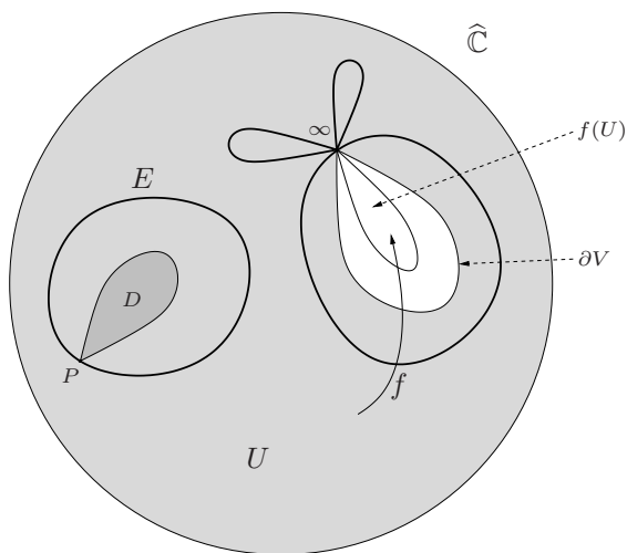
Figure 3.18: If there exists a pole P on \partial E , then there exists a set D \subset E such that f(D) = V , where V is an unbounded simply-connected set that contains U but not f(U) . The thick lines correspond to \partial U , while the sets D and V appear dark- and light-shaded, respectively.
