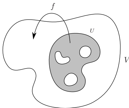
Figure 2.2: A rational-like map in the special case of V simply connected.
