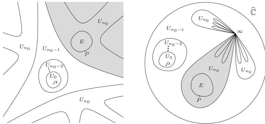
Figure 3.11: The increasing sequence of open sets \{U_k\}_k and the decreasing one \{V_k\}_k . In this example, U_{n_0-1} is the first unbounded set in the sequence and, consequently, V_n = \widehat{\mathbb{C}} \setminus U_n for all n < n_0 - 1 . The shaded set corresponds to V_{n_0-1} , while V_{n_0} = E . The same situation has been drawn on the plane and on the Riemann sphere.
