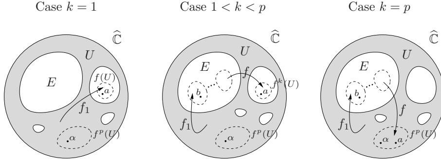
Figure 3.7: The topological surgery construction for the three possible cases, drawn on \widehat{\mathbb{C}} .
