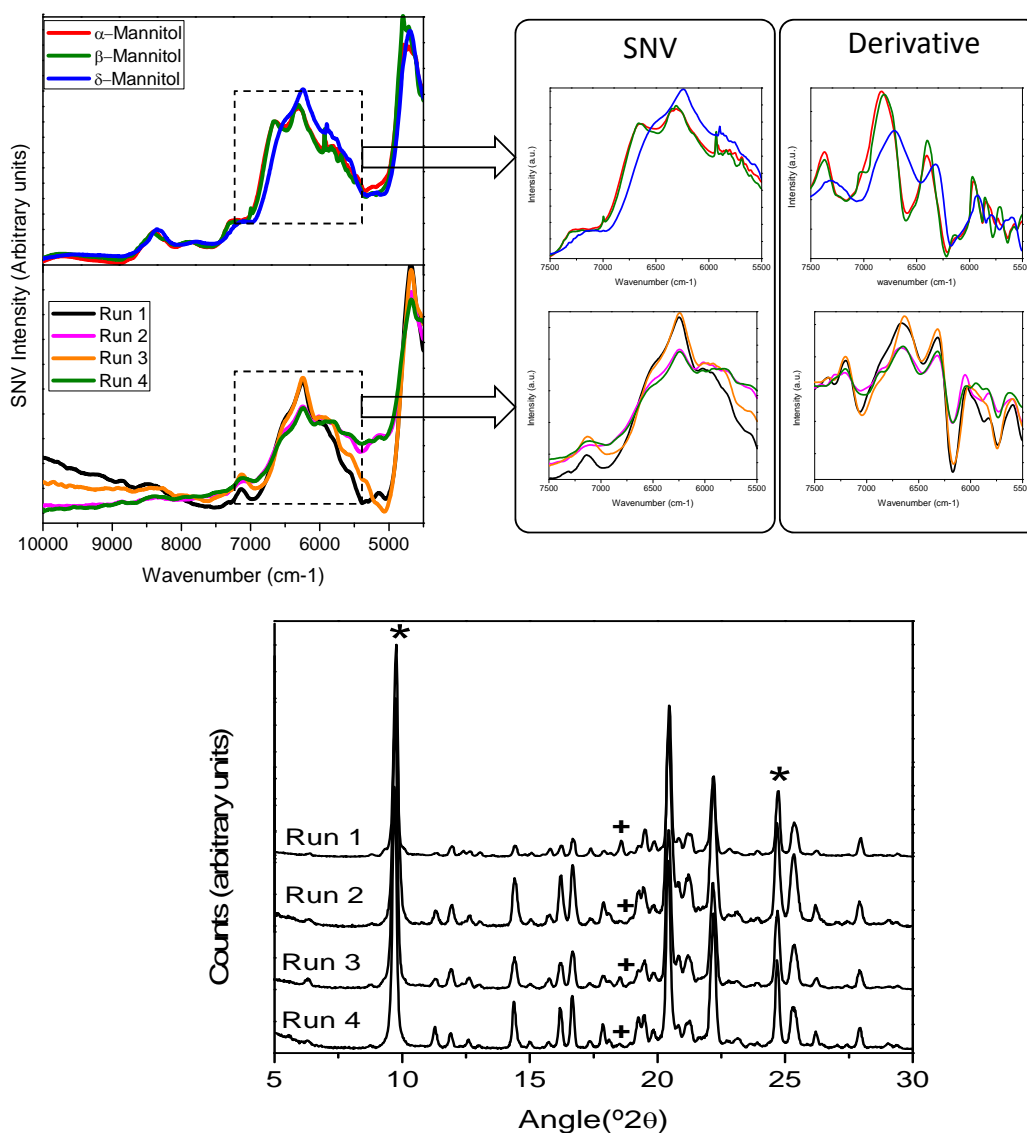
Figure 3. Physicochemical characterization of mannitol polymorph in end-products. a) and c) NIR spectra of \alpha -, \beta -, and \delta -mannitol polymorphs in SNV and 1st derivative mode, respectively. b) and d) NIR spectra of end-products for each experiment in SNV and 1st derivative mode, respectively, and e) XRPD of end-products (*) and (+) characteristic diffractions for \delta - and hemihydrate mannitol, respectively.
