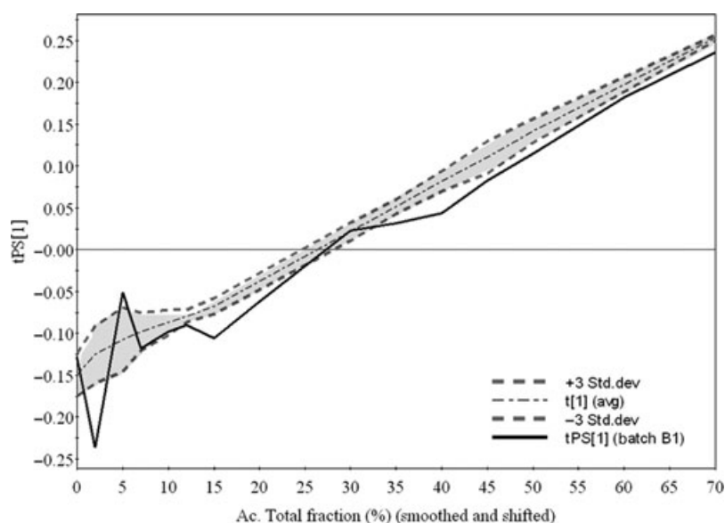
Figure 7. Control charts for the scores of a model constructed from NIR spectra.
