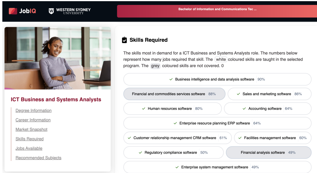
Figure 5.7: Screenshot of JobIQ showing the skills required by the ICT Business and Systems Analysts job and which skills are acquired after completing the Bachelor’s Degree in ICT.
