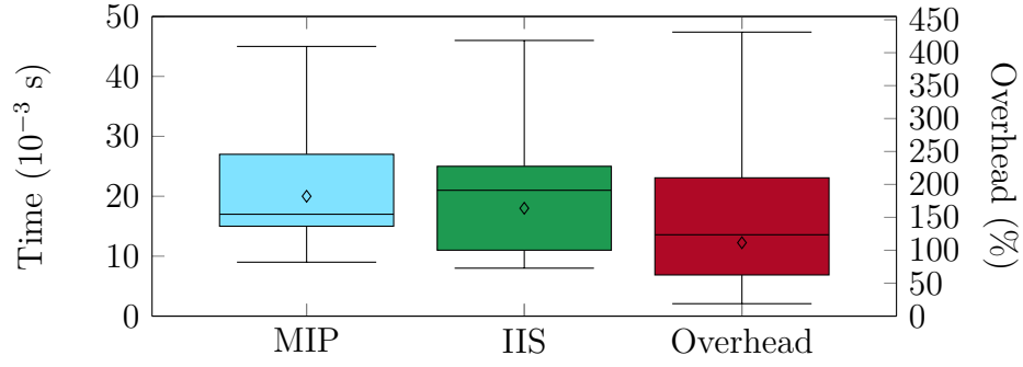
Figure 7.2: Runtimes to solve the MIP problem and compute IIS (left y-axis), and time overhead (right y-axis), for DPP.
