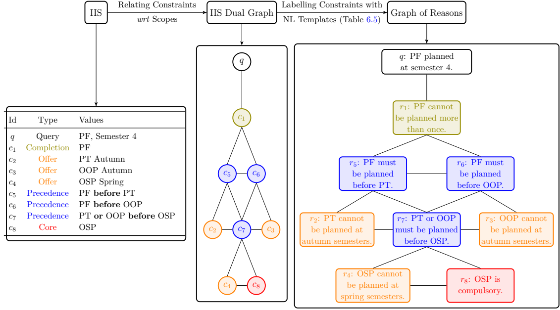
Figure 6.2: Process to build a graph of reasons applied to our running example: (1) relating constraints within the IIS to yield its dual graph, and (2) labelling constraints in the dual graph to build the graph of reasons.
