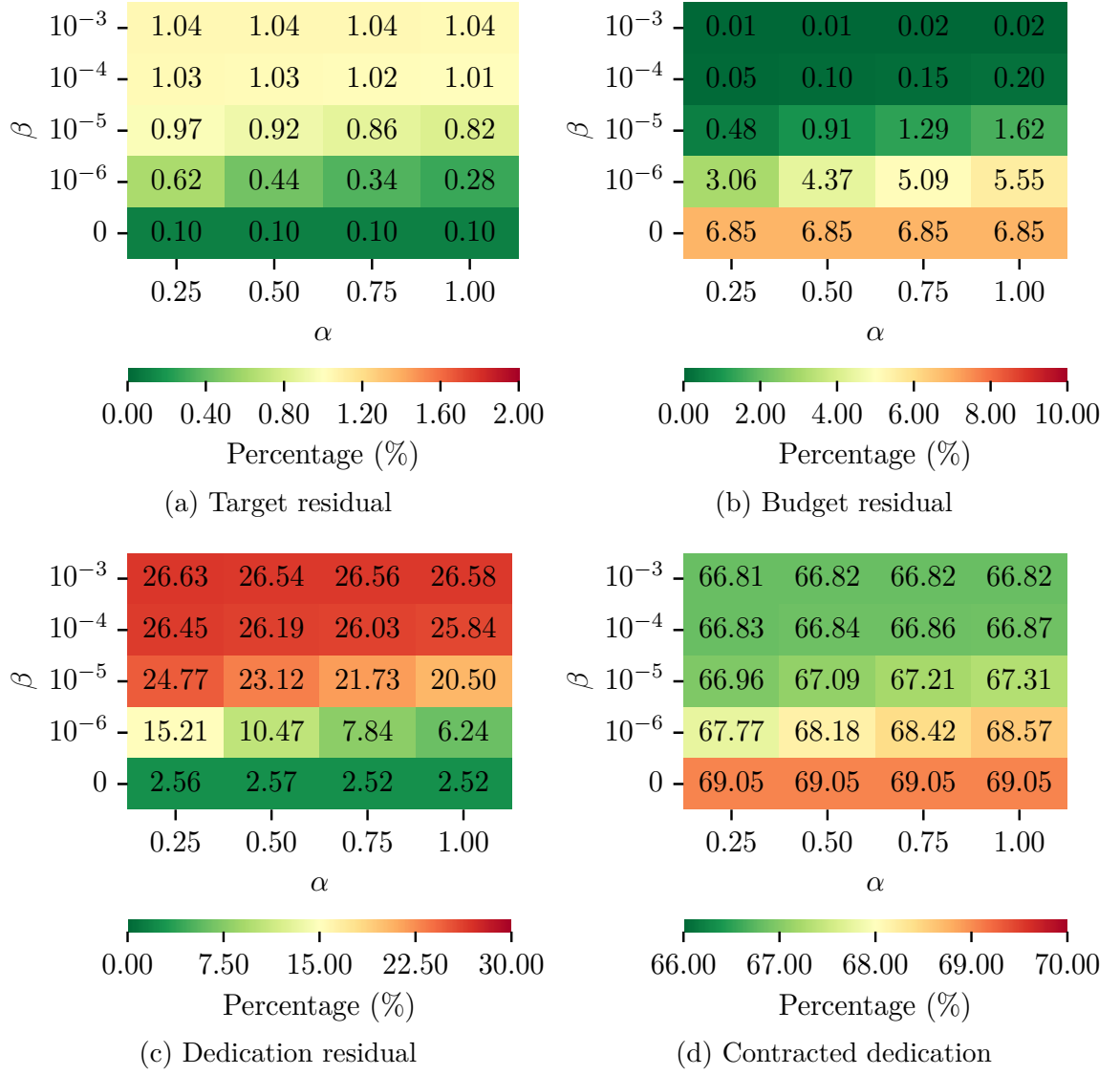
Figure 4.2: Results in the abundant budget scenario for \gamma = \infty .
