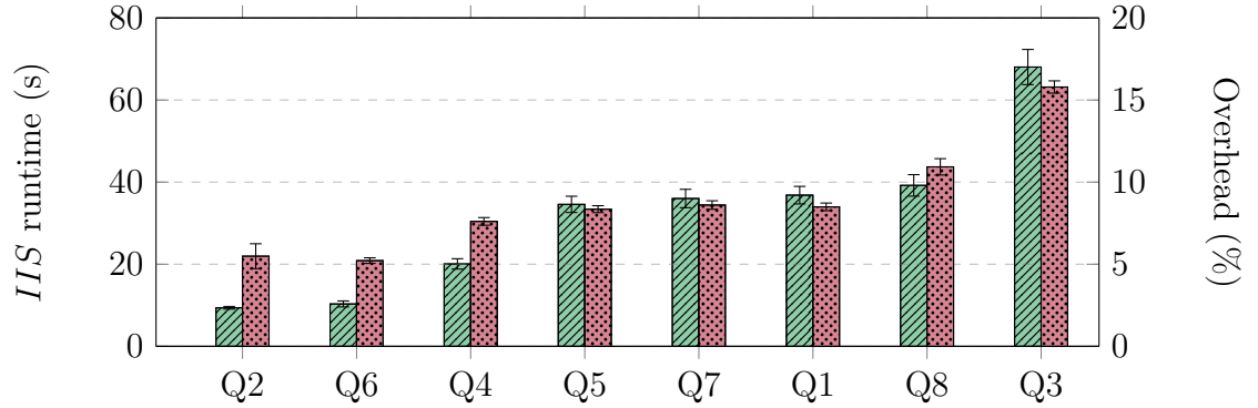
Figure 7.8: Average IIS computation time (lines, left y-axis) and overhead (dots, right y-axis) for different query types for the RCPSP.
