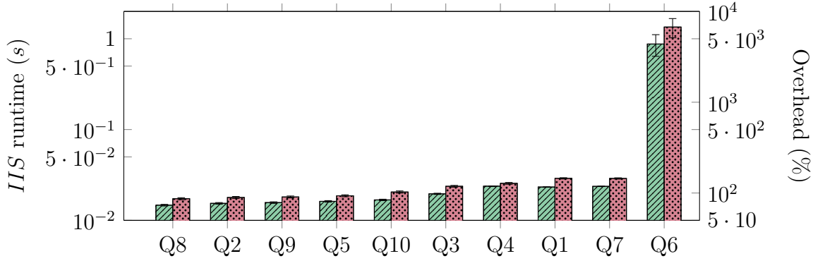
Figure 7.3: Average IIS computation time (lines, left y-axis) and overhead (dots, right y-axis) for different query types for the DPP.
