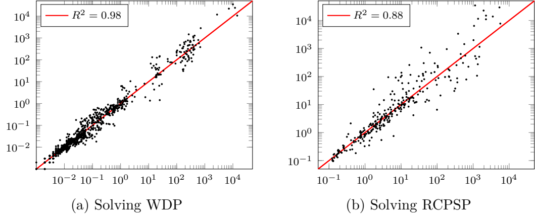
Figure C.1: Solving time predictions on previously unseen test instances for Random Forest (best performing model). The x -axis denotes the runtime prediction, and the y -axis denotes the real runtime. Each data point represents one instance. We show the Coefficient of Determination ( R^2 ), which measures how well the model predicts runtime (1 indicates a perfect fit).
