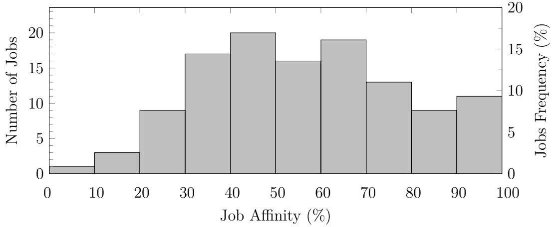
Figure 5.2: Histogram of job affinities for all jobs. We report the distribution of the job affinity values in two frequency metrics: the absolute number of jobs (left axis), and the percentage of jobs (right axis).
