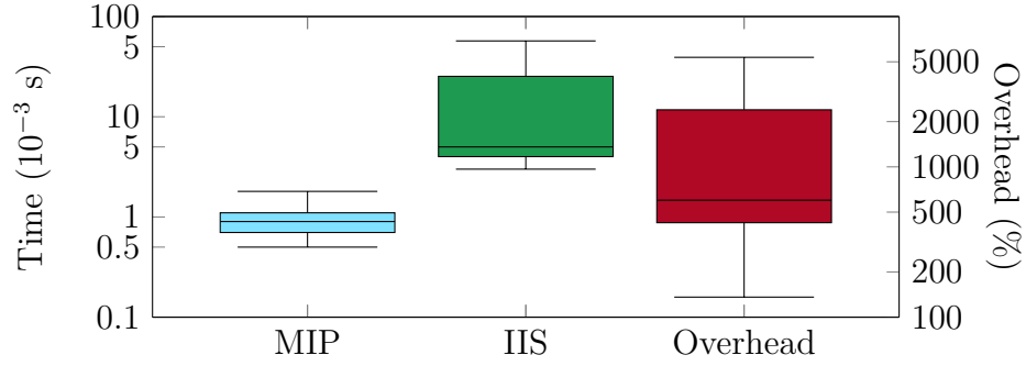
Figure 7.6: Runtimes to solve the optimisation problem and compute IIS (left y-axis), and time overhead (right y-axis), for the aggregation of value systems.
