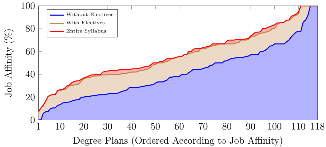
Figure 5.4: Cactus plot showing the job affinity for the degree plan of each target job. We order degree plans from the lowest job affinity to the highest on the x-axis. We plot the job affinity considering degree plans without the elective units (in blue); whole degree plans (in brown); and all units from the degree syllabus, \mathcal{U} (in red).
