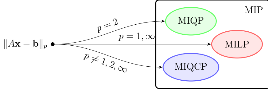
Figure 2.2: Subclasses of MIPs and p -norm minimisation problems depending on the value of p .
