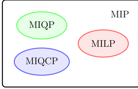
Figure 1.2: Classes of MIP problems. While MILPs consider linear objective and constraints, MIQP considers a quadratic objective function, and MIQCP comprise problems with quadratic constraints.
