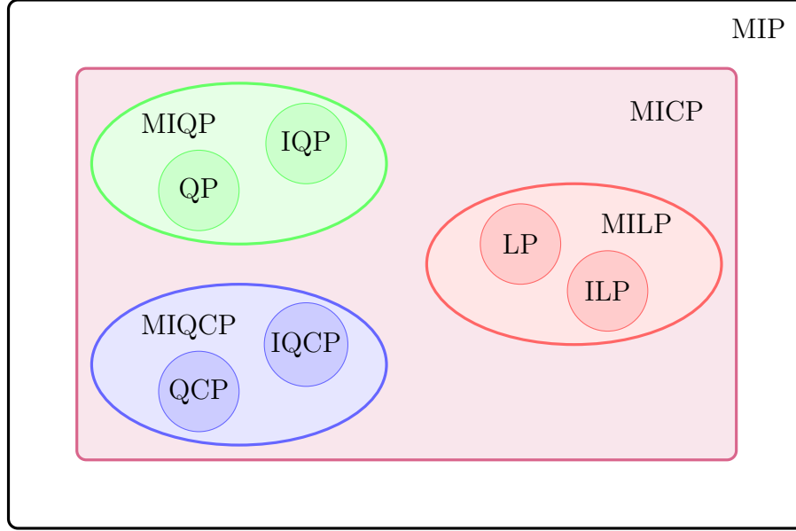
Figure 2.1: Classes of MIP problems. In particular, MILP, MIQP, and MIQCP can be further divided into two subclasses: those with only discrete variables, such as ILP, IQP, and IQCP, and those with only continuous variables, such as LP, QP, and QCP. MILP, MIQP, and MIQCP are specific cases of MICP.
