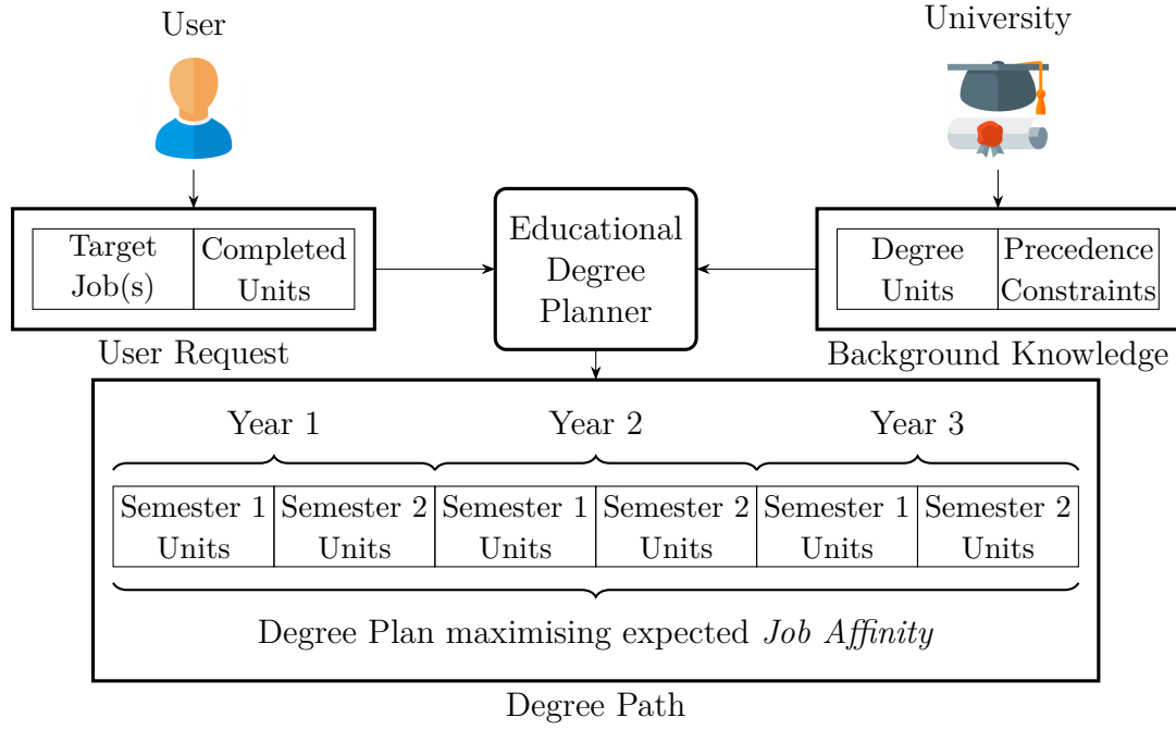
Figure 5.1: Overview of our automated solution approach. We refer the reader to Sections 5.2 and 5.3 for the technical details.
