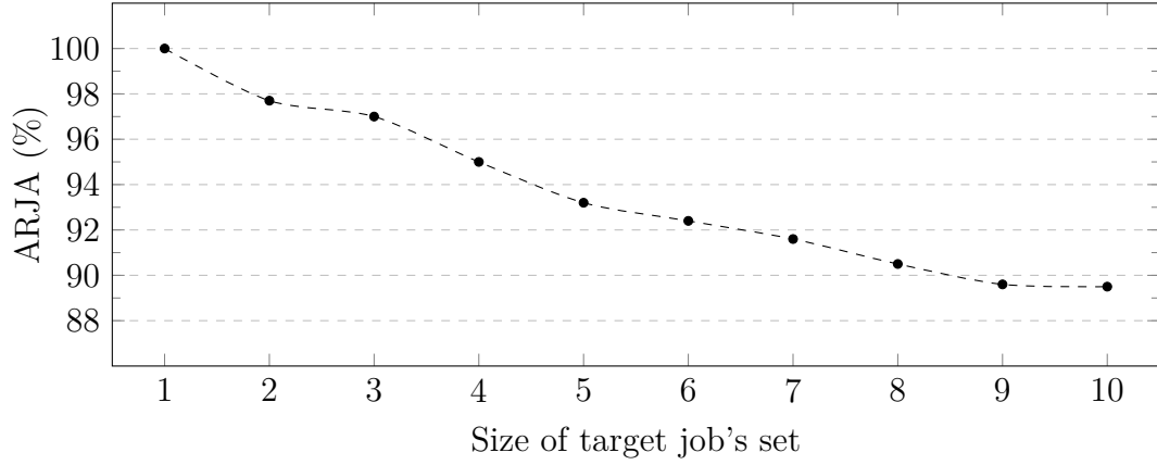
Figure 5.5: Average RJA along the size of the set of target jobs.
