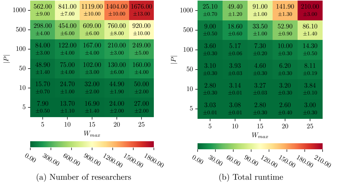
Figure 4.4: Fig. 4.4a reports the number of researchers generated with respect to the number of projects |P| and the maximum number of work packages per project W_{max} . Fig. 4.4b reports the total solution runtime. Each cell reports the average and the standard error of the mean over the 10 instances generated for each combination of |P| and W_{max} .
