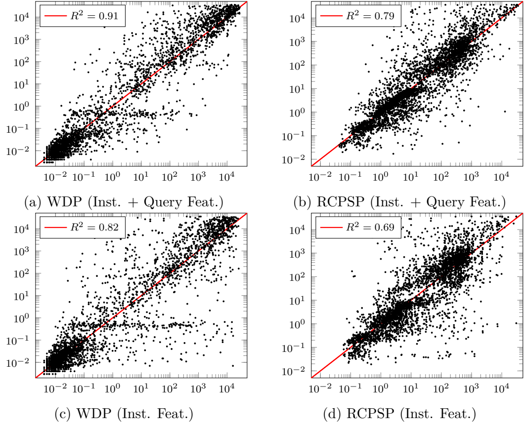
Figure 7.10: IIS Runtime predictions on previously unseen test instances for Random Forest (best performing model). The x -axis denotes the runtime prediction, and the y -axis denotes the real runtime. Each data point represents one instance. We show the Coefficient of Determination ( R^2 ), which measures how well the model predicts runtime (1 indicates a perfect fit).
