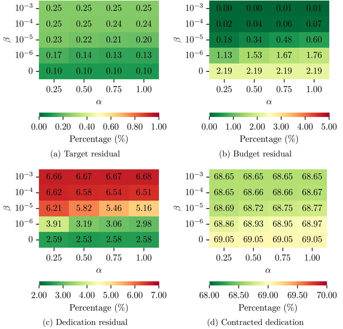
Figure 4.1: Results in the sufficient budget scenario for \gamma = \infty (best viewed in colours).
