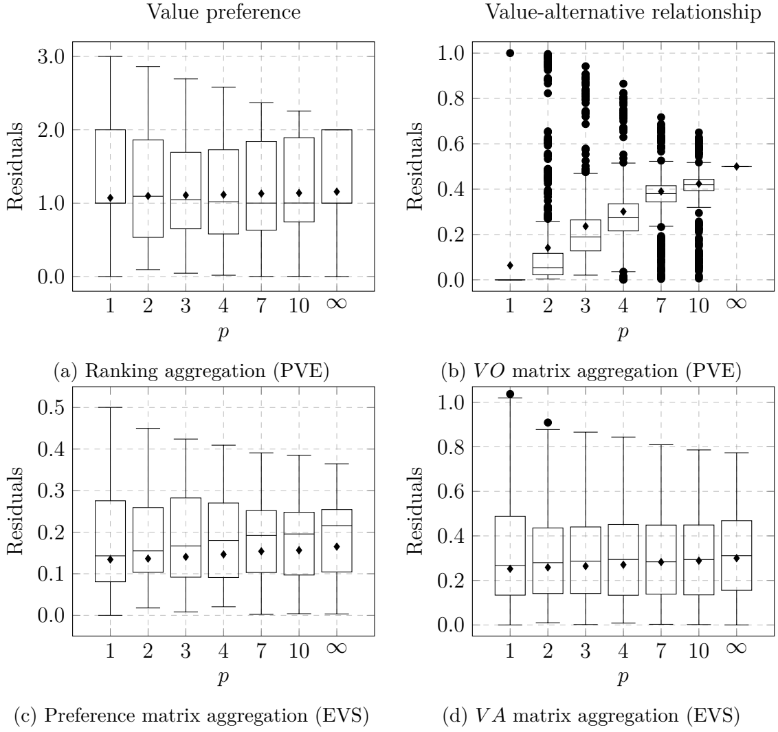
Figure 3.3: Boxplots of residuals for different ethical principles in the value preference and value-alternative aggregation for the PVE (top) and EVS (bottom) case study. The diamond represents the mean and the circles represent the outliers.
