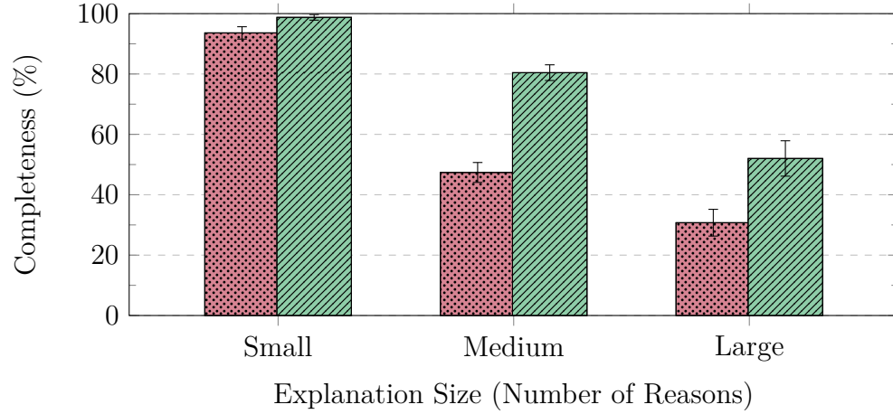
Figure 6.3: Average percentage of reasons mentioned in the explanations generated using the IIS (red) and using the graph of reasons (green). We group the explanations into three groups depending on the number of reasons: (i) small (less than five reasons), (ii) medium (between five and ten reasons), and (iii) large (more than ten reasons).
