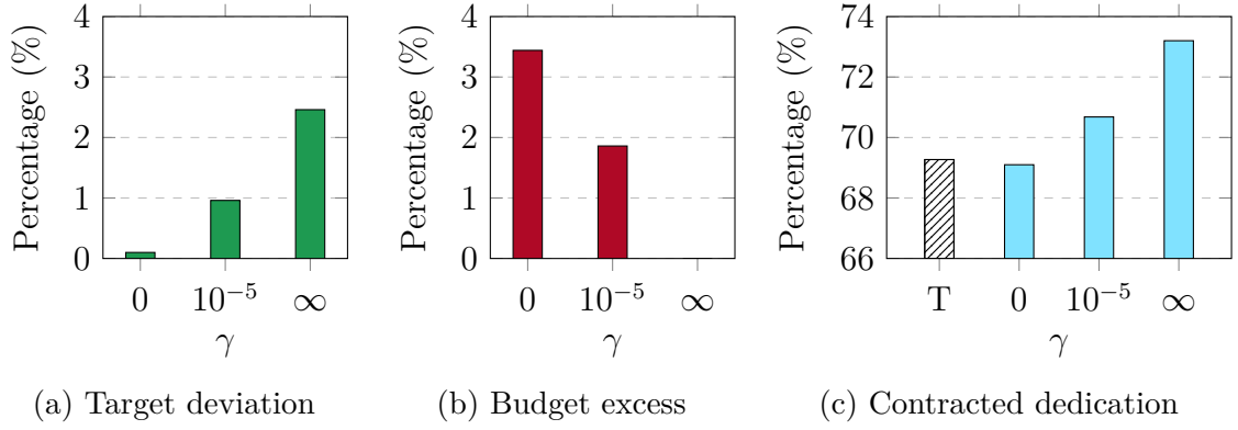
Figure 4.3: Target deviation (4.3a), budget excess (4.3b), and comparison between the contracted researchers' dedication with their target (4.3c), for different \gamma and for \alpha = 0.25 , \beta = 0 .
