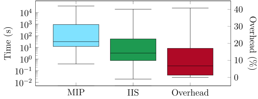
Figure 7.7: Boxplot of the Solving time of the MIP problem, the IIS runtime (left y axis), and the Overhead for the RCPSP (right y axis).
