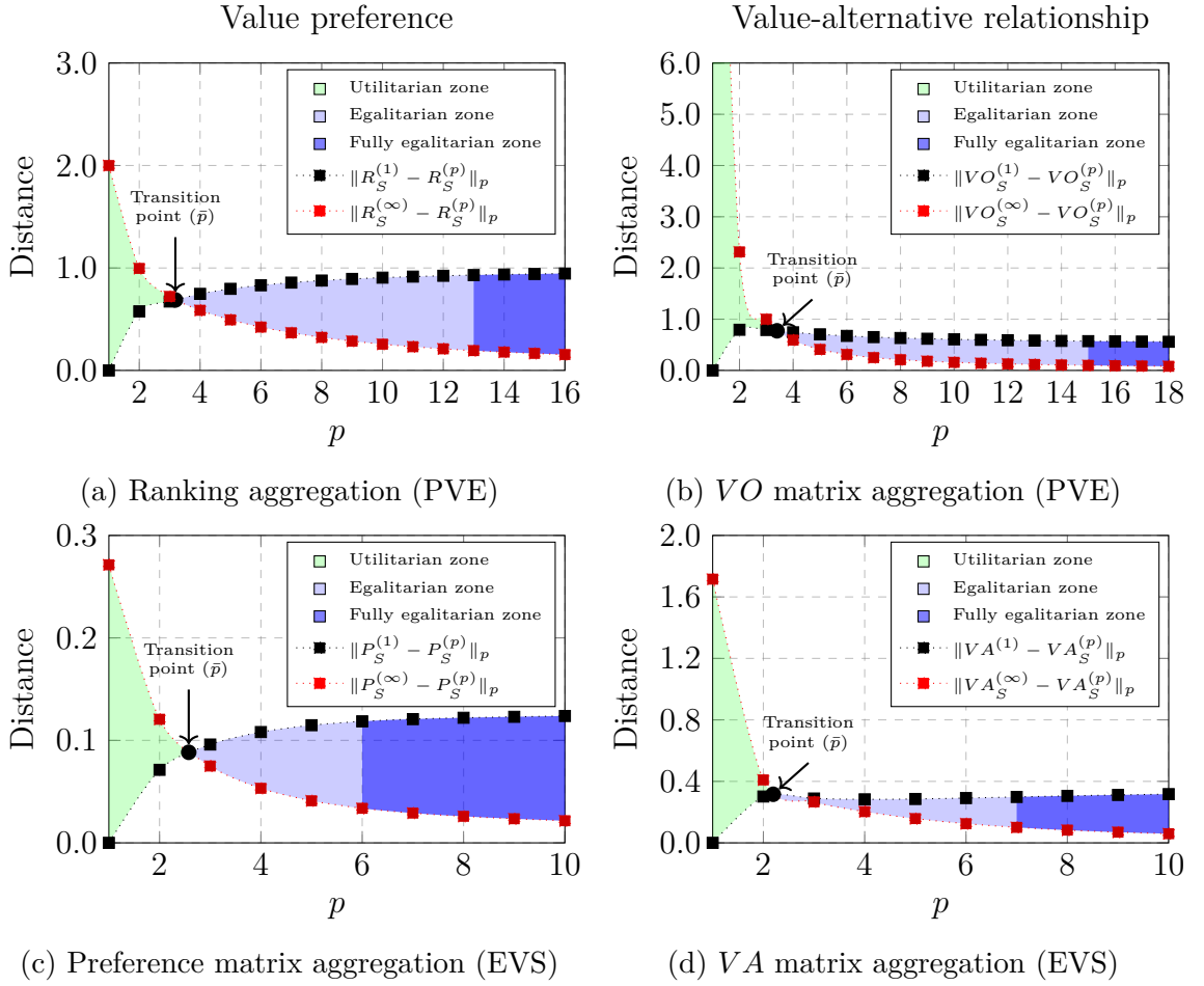
Figure 3.2: Distance between the consensus computed according to ethical principle p and the consensus computed according to p = 1 (fully utilitarian, black line) and p = \infty (fully egalitarian, red line). The transition point \bar{p} is the ethical principle producing a consensus equidistant from the fully utilitarian and fully egalitarian ones. Thus, \bar{p} divides the space of ethical principles into an utilitarian zone (more similar to the fully utilitarian consensus, green) and an egalitarian zone (more similar to the fully egalitarian consensus, light blue). The fully egalitarian (dark blue) zone marks the ethical principles that produce a consensus approximately equal (to a small \epsilon ) to the fully egalitarian one. PVE case study on top, and EVS case study for the population-based influence case at the bottom.
