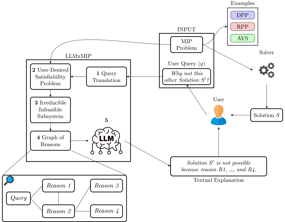
Figure 6.1: Overview of our explanatory approach. Section 6.2 discusses its steps in detail.
