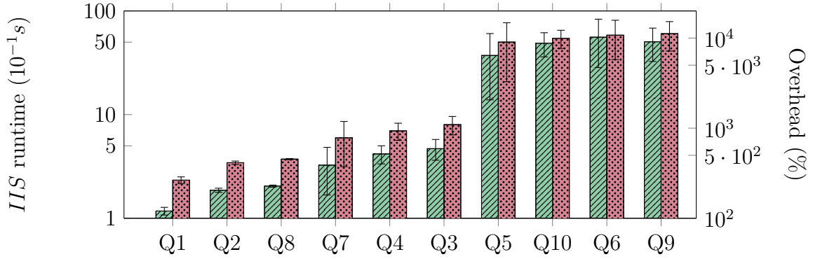
Figure 7.5: Average IIS computation time (lines, left y-axis) and overhead (dots, right y-axis) for different query types for the RPP problem.
