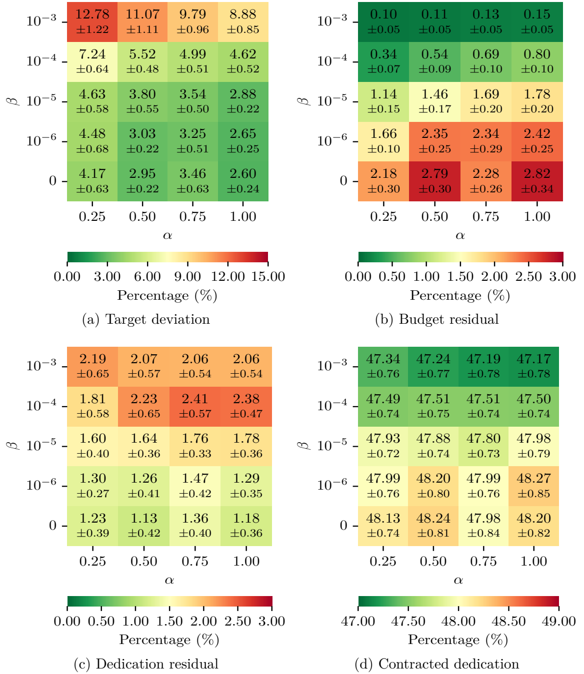
Figure 4.5: Results in the sufficient budget scenario for \gamma = \infty considering uncertainty.
