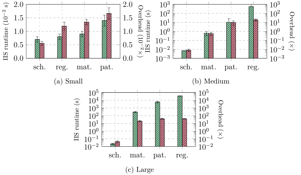
Figure 7.9: Average IIS runtimes (lines) and overhead (dots) for different WDP instance distributions: scheduling , matching , paths , and regions .
