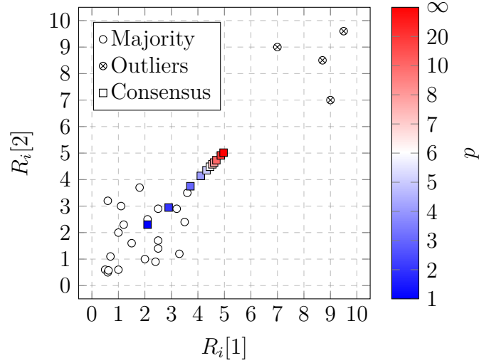
Figure 3.1: The impact of the ethical principle p on the computed consensus of a set of individuals' judgement of two objects: R_i[1] and R_i[2] . Circles show the individuals' judgement and squares represent the consensus computed. Squares are filled with the colour of the ethical principle used to compute the consensus. (Best viewed in colour).
