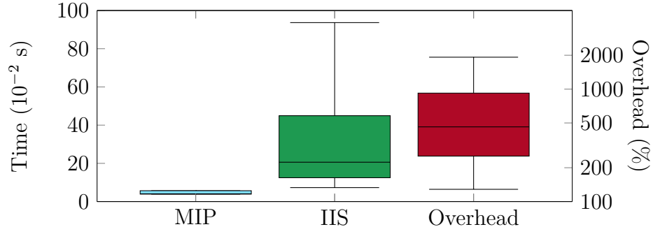
Figure 7.4: Runtimes to solve the MIP problem and compute IIS (left y-axis), and time overhead (right y-axis), for the RPP problem.
