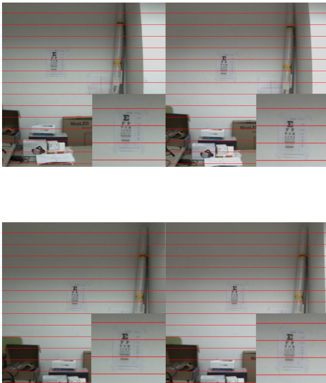
Fig. 11: On top there is an example of one image pair as it is captured from the cameras. In these images the objects cannot be found on the same Y scanline. This can be noticed on the pattern in the middle of the image. On bottom the same images from the top have been rectified using the calibration module. The distortion, the rotation and the translation produced by the camera are gone and the objects can be found in the same Y scanline.
