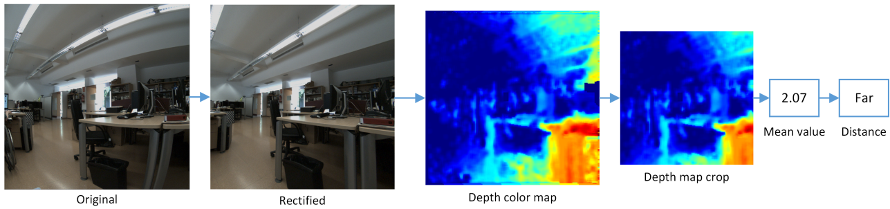
Fig. 5: Example of the transformations applied to a far distance image to get the distance class.
