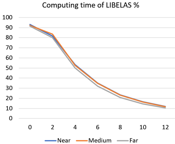
Fig. 6: Computing time of LIBELAS in percentage over the total processing time in 3 different videos with different distances.
