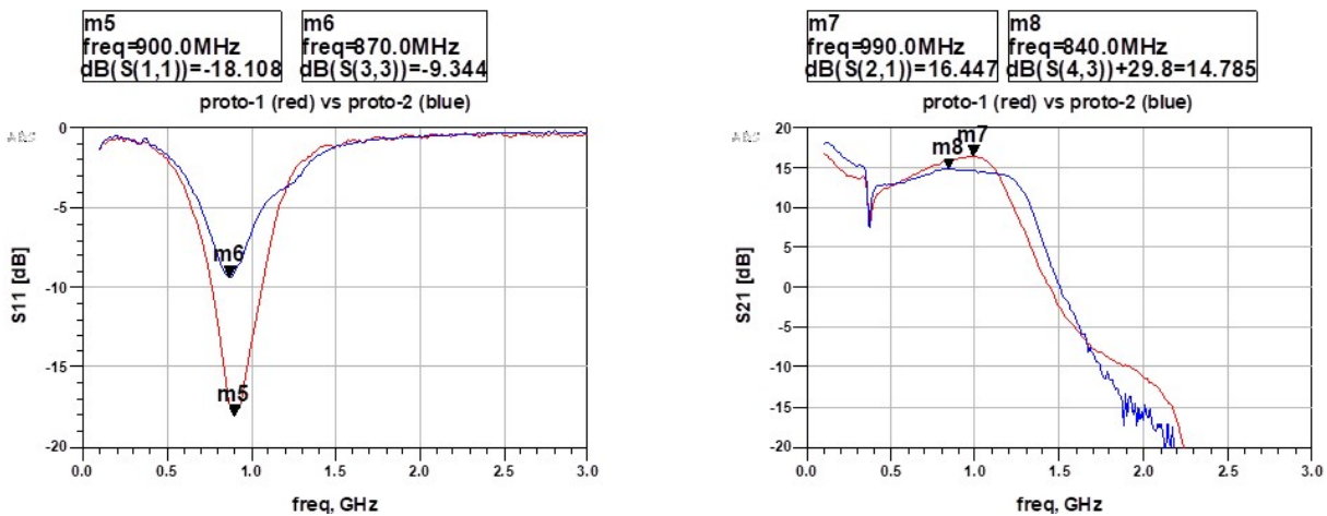
Figure 4.11: Small signal measurement: Prototype 1 vs Prototype 2
