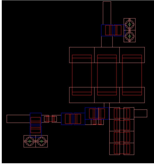
Figure 3.15: Input network considering Resistors deratings
