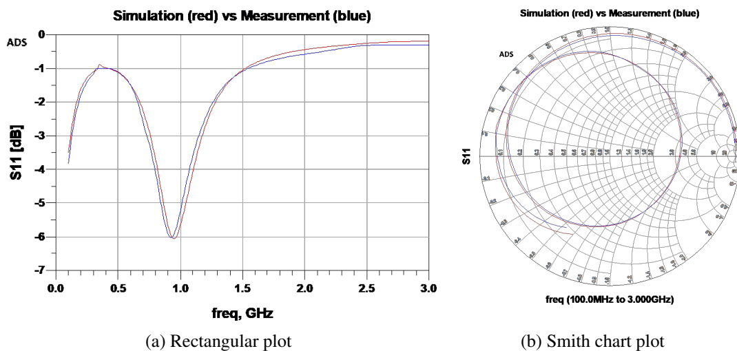
Figure 5.18: Input passive network correlation (figure 4.12) S-parameters
