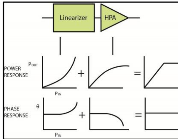
Figure 1.1: Linearizer [1]
