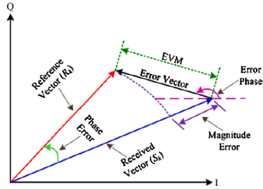
(c) Illustration of error vector magnitude (EVM) and its components
