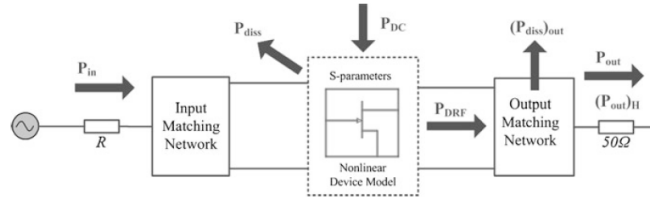
(b) Power flow depiction in a power amplifier [3]
