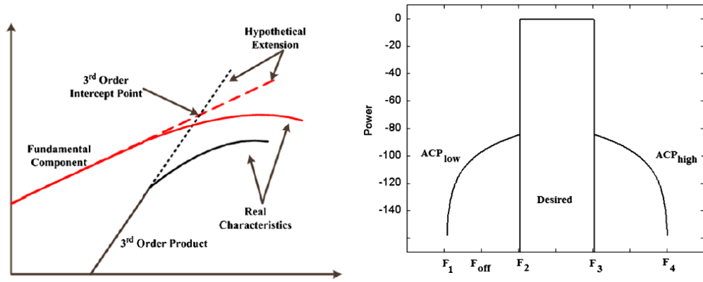
(a) Representation of third-order intercepts point (b) Ideal representation of main and adjacent channel power spectra and their respective frequency band definitions
