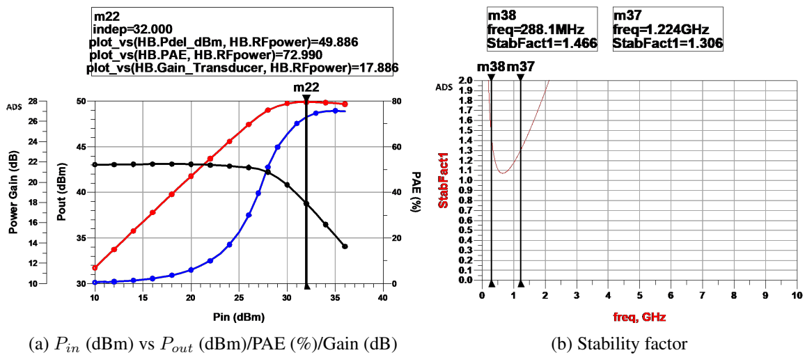
Figure 3.9: Harmonic Balance Simulation performance including stability network
