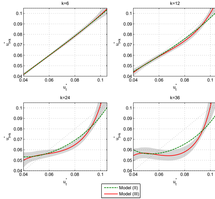
Figure A12: Specification for the job loss rate
