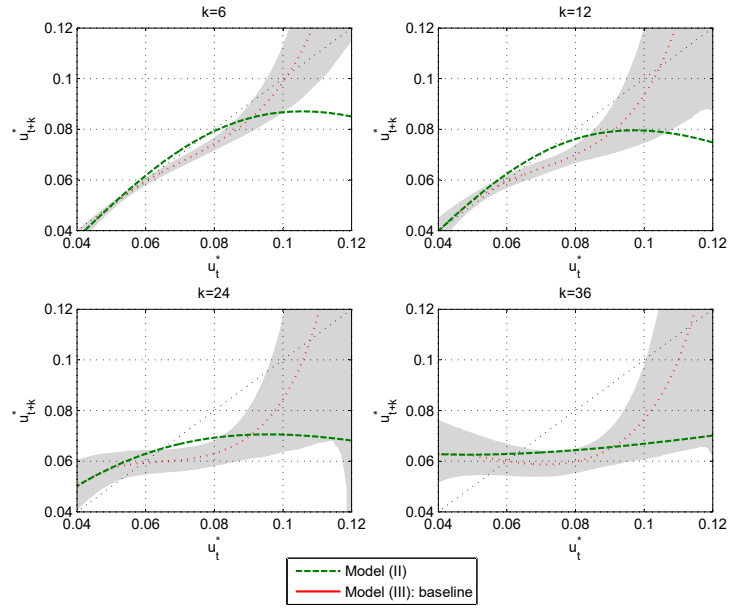
Figure A6: Conditional density of u_{t+k}^* given u_t^* for duration-based CPS data (1970-2015)
