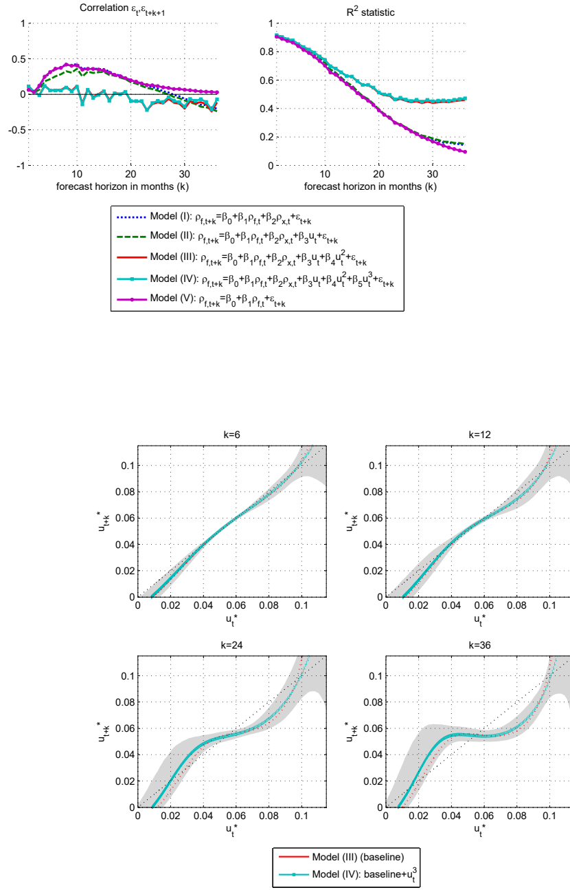
Figure A1: Diagnostics statistics: additional higher-order terms and AR(1)
